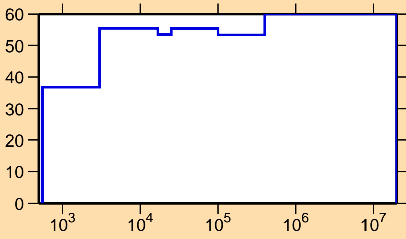
\Delta\sigma/\sigma vs. E for ^{160}\text{Hf}(n,\gamma)
