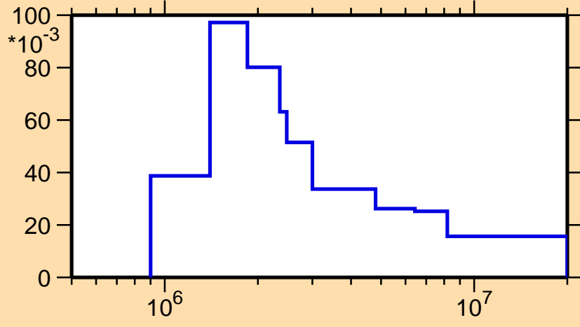
\sigma vs. E for ^{160}\text{Hf}(n,n_2)
