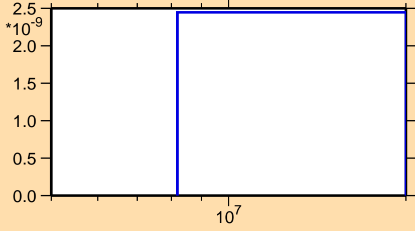
\sigma vs. E for ^{160}\text{Hf}(n,\text{nd})
