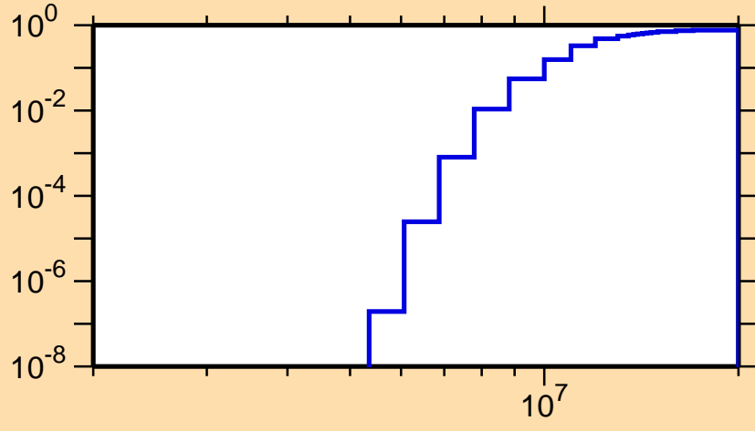
\sigma vs. E for ^{161}\text{Hf}(n,np)
