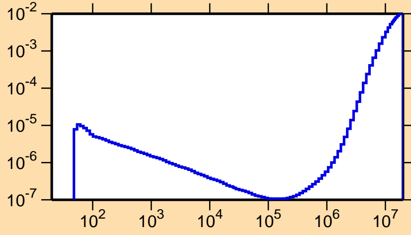
\sigma vs. E for ^{161}\text{Hf}(n,p\alpha)
