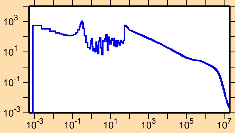
\sigma vs. E for ^{161}\text{Hf}(n,\gamma)
