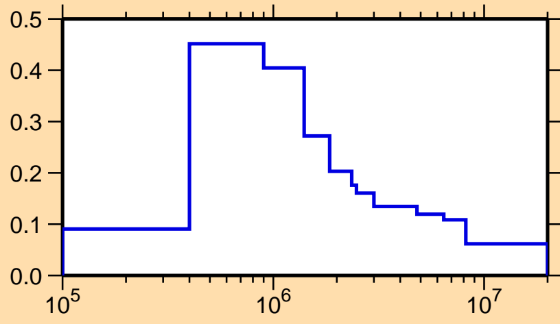
\sigma vs. E for ^{161}\text{Hf}(n,n_1)
