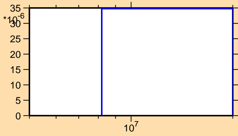
\sigma vs. E for ^{162}\text{Hf}(n,t)
