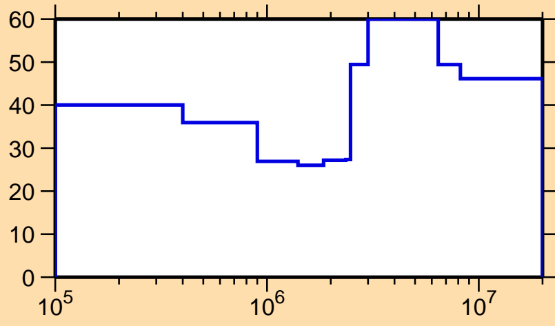
\Delta\sigma/\sigma vs. E for ^{162}\text{Hf}(n,n_1)
