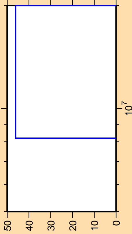
\Delta\sigma/\sigma vs. E for ^{162}\text{Hf}(n,n_1)
