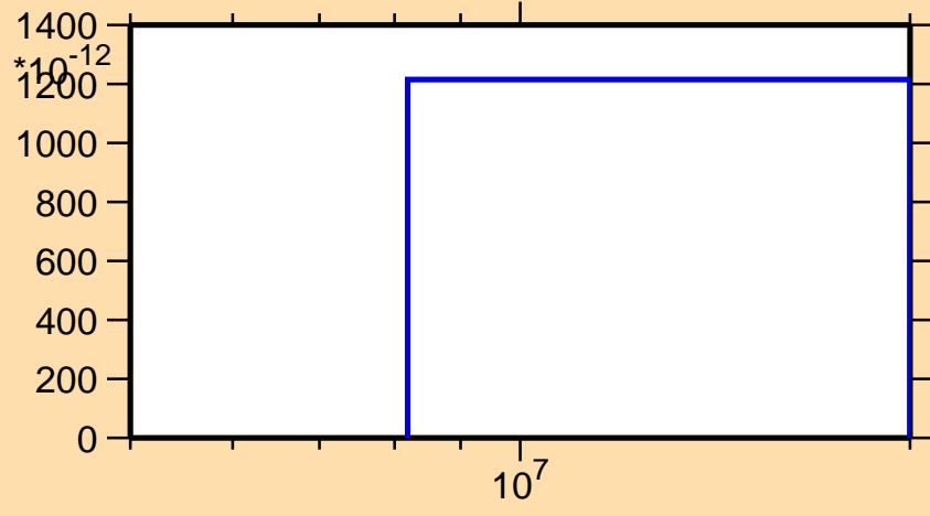
\sigma vs. E for ^{162}\text{Hf}(n,nd)
