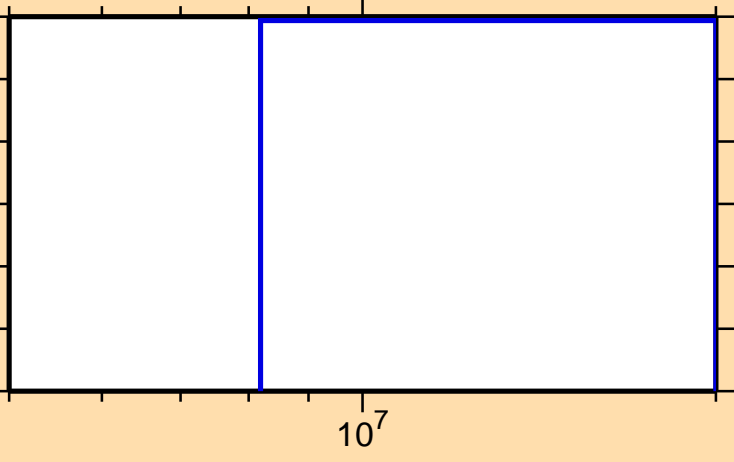
\sigma vs. E for ^{162}\text{Hf}(n,3n)
