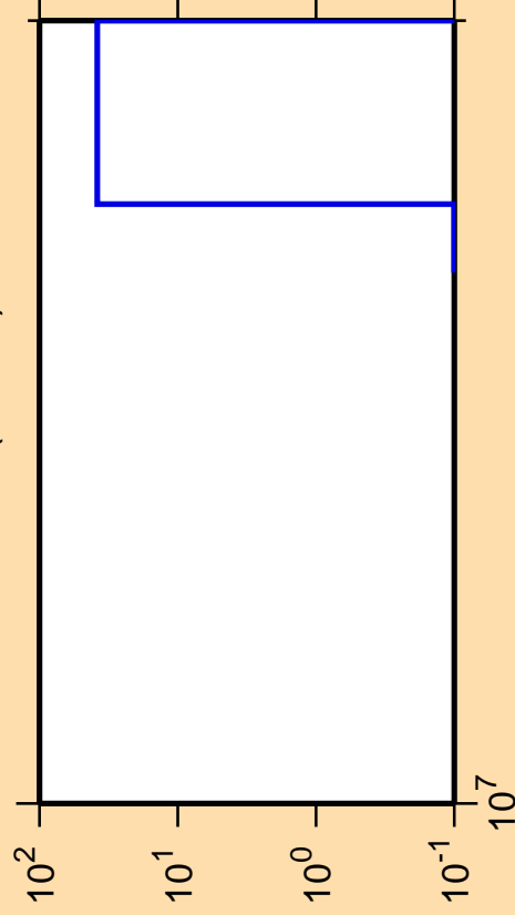
\Delta\sigma/\sigma vs. E for ^{163}\text{Hf}(n,3n\alpha)
