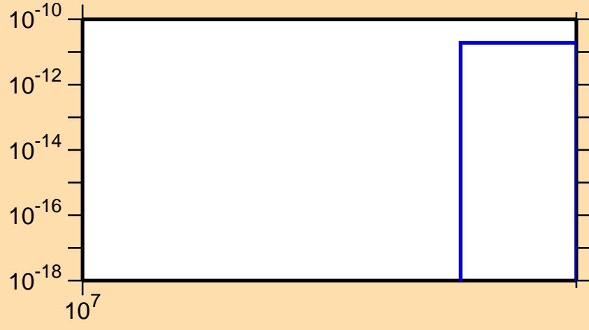
\sigma vs. E for ^{163}\text{Hf}(n,3n\alpha)
