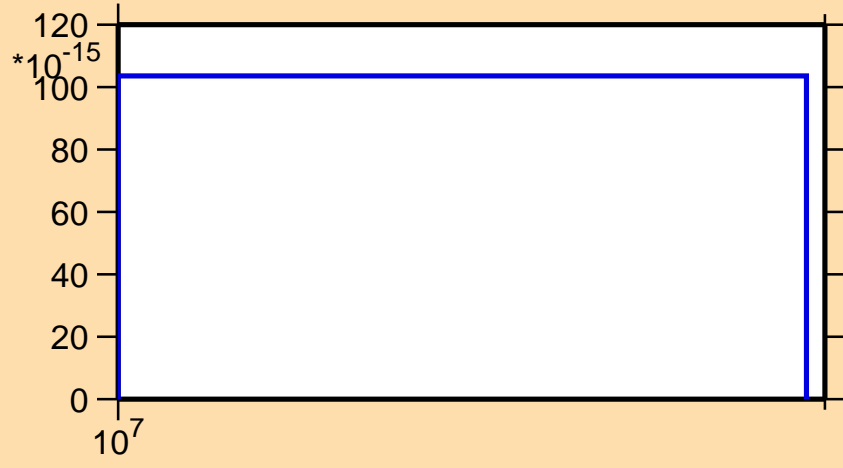
\sigma vs. E for ^{163}\text{Hf}(n,3n\alpha)
