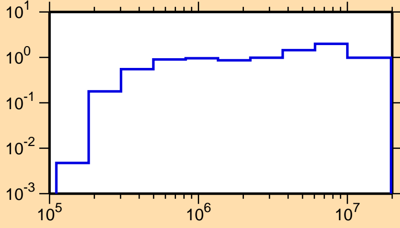
\sigma vs. E for ^{163}\text{Hf}(n,\text{inel.})
