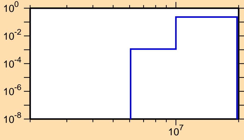
\sigma vs. E for ^{163}\text{Hf}(n,np)
