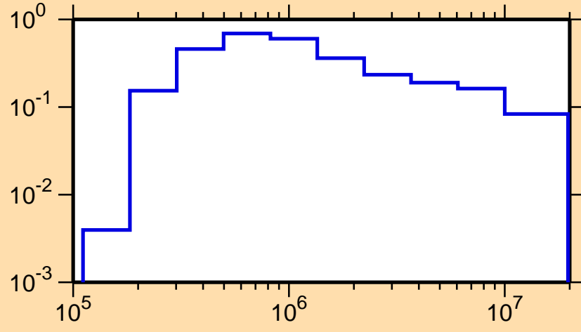
\sigma vs. E for ^{163}\text{Hf}(n,n_1)
