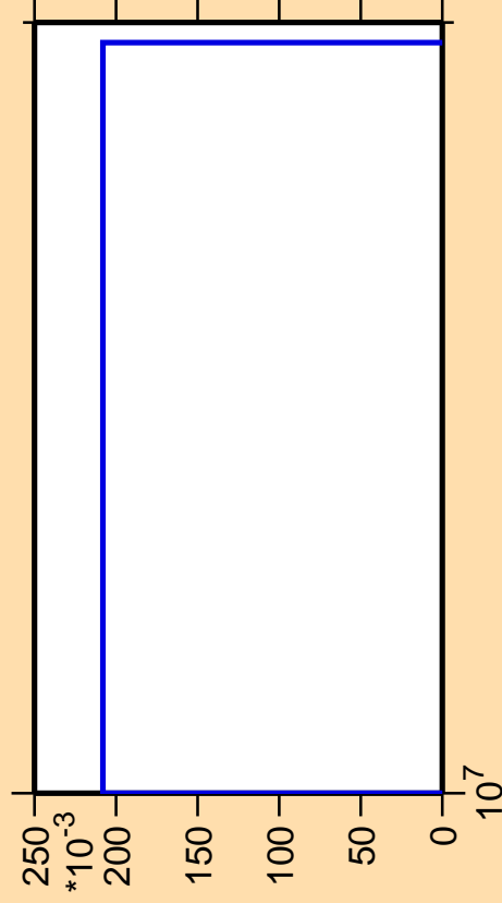
\Delta\sigma/\sigma vs. E for ^{163}\text{Hf}(n,3n\alpha)
