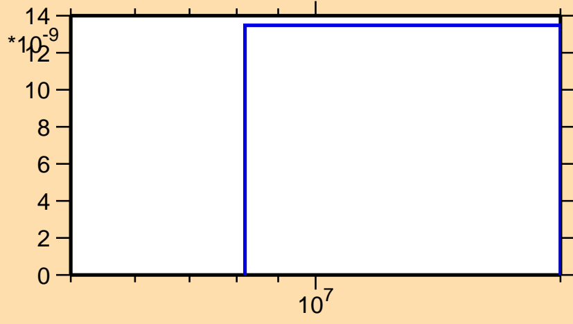
\sigma vs. E for ^{163}\text{Hf}(\text{mt117})
