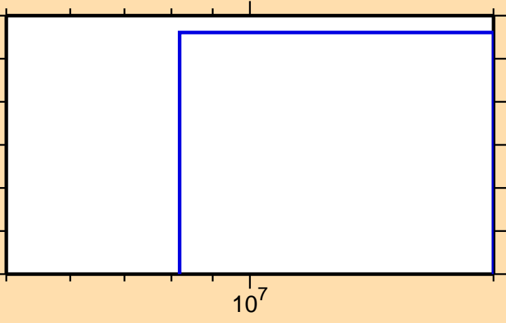
\sigma vs. E for ^{163}\text{Hf}(n,\text{nd})
