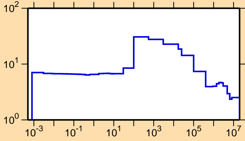
\sigma vs. E for ^{163}\text{Hf}(n,\text{el.})
