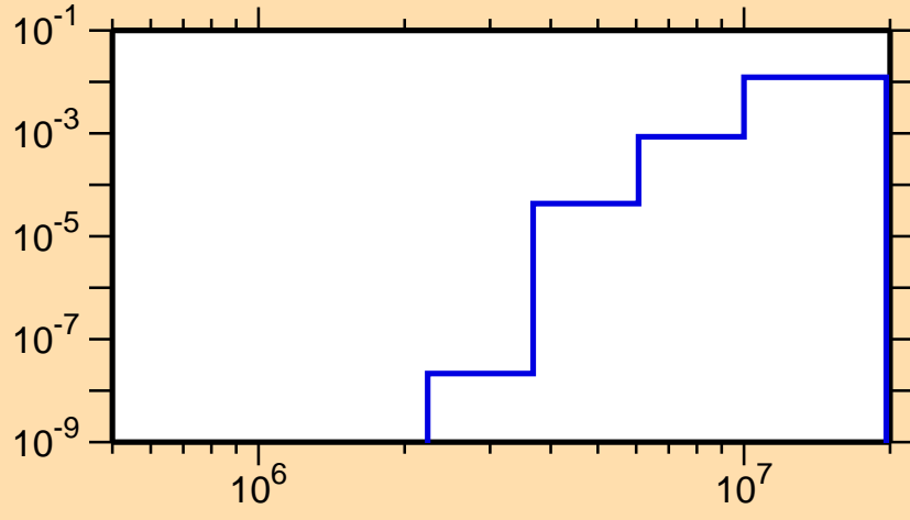
\sigma vs. E for ^{164}\text{Hf}(n,n\alpha)
