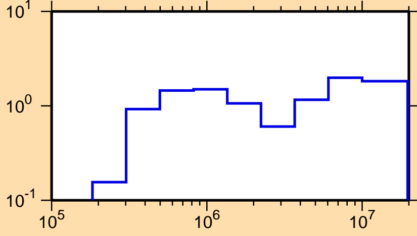
\sigma vs. E for ^{164}\text{Hf}(n,\text{inel.})
