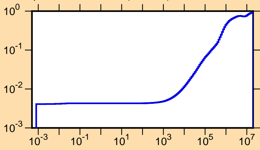
\mu vs. E for ^{165}\text{Hf(mt251)}
