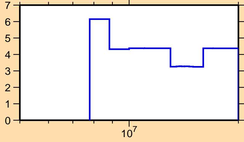
\Delta\sigma/\sigma vs. E for ^{165}\text{Hf}(n,\text{tot.})
