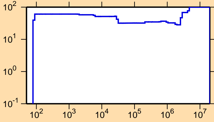
\Delta\sigma/\sigma vs. E for ^{165}\text{Hf}(n,\gamma)
