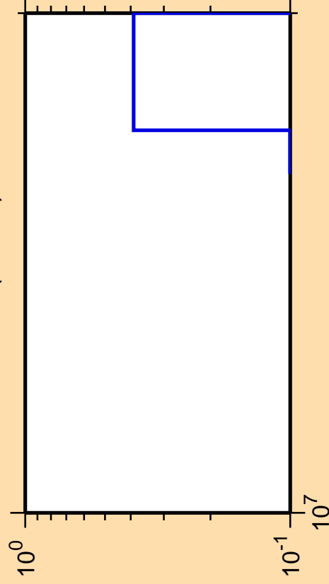
\Delta\sigma/\sigma vs. E for ^{165}\text{Hf}(n,3n\alpha)
