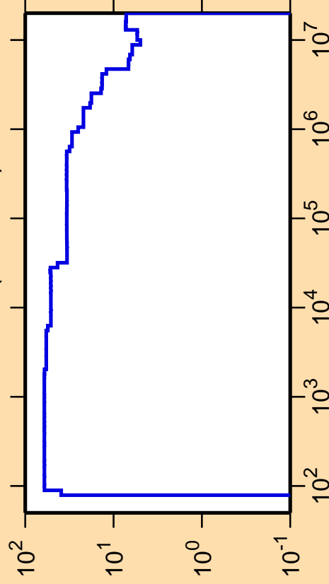
\Delta\sigma/\sigma vs. E for ^{165}\text{Hf}(n,\text{nonel.})
