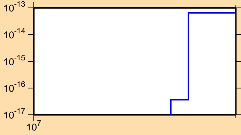
\sigma vs. E for ^{165}\text{Hf}(n,3n\alpha)
