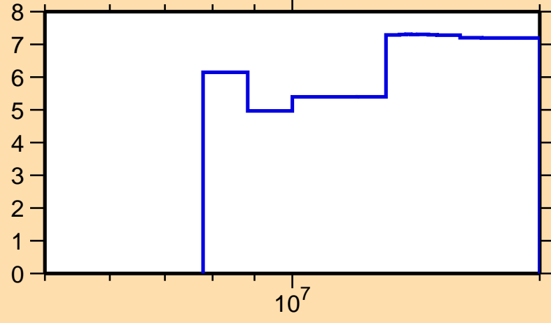
\Delta\sigma/\sigma vs. E for ^{165}\text{Hf}(n,\text{nonel.})
