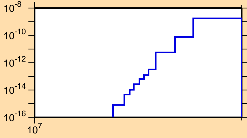
\sigma vs. E for ^{165}\text{Hf}(\text{mt } 34)
