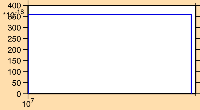
\sigma vs. E for ^{165}\text{Hf}(n,3n\alpha)
