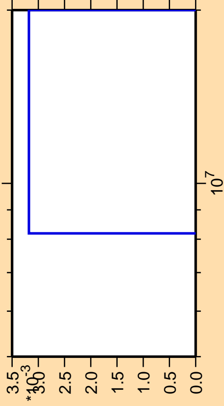
\Delta\sigma/\sigma vs. E for ^{165}\text{Hf}(n,3n\alpha)
