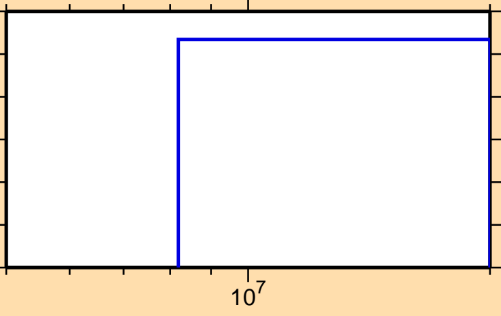
\sigma vs. E for ^{165}\text{Hf}(n,3n\alpha)
