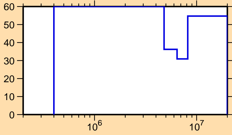
\Delta\sigma/\sigma vs. E for ^{165}\text{Hf}(n,n\text{cont.})
