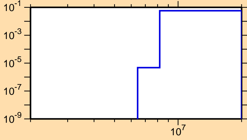
\sigma vs. E for ^{165}\text{Hf}(n,np)
