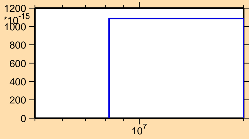
\sigma vs. E for ^{165}\text{Hf}(n,nt)
