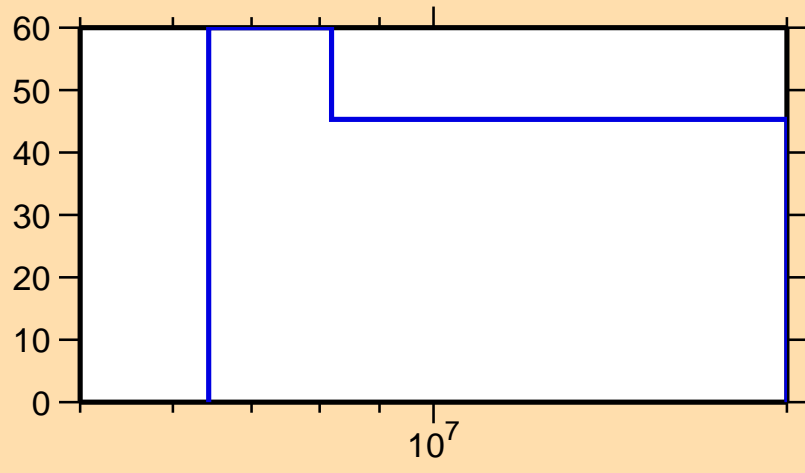
\Delta\sigma/\sigma vs. E for ^{165}\text{Hf}(n,2n)
