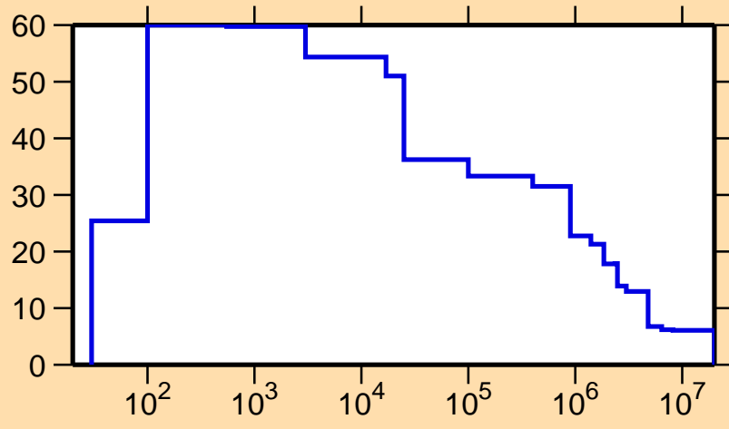
\Delta\sigma/\sigma vs. E for ^{165}\text{Hf}(n,\text{nonel.})
