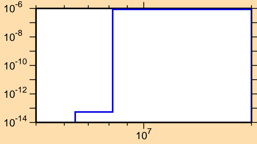
\sigma vs. E for ^{165}\text{Hf}(n,\text{He3})
