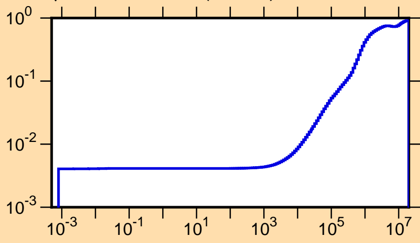
\mu vs. E for ^{166}\text{Hf(mt251)}
