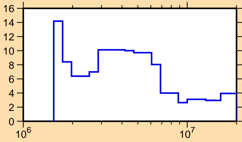
\Delta\sigma/\sigma vs. E for ^{166}\text{Hf}(n,\text{tot.})
