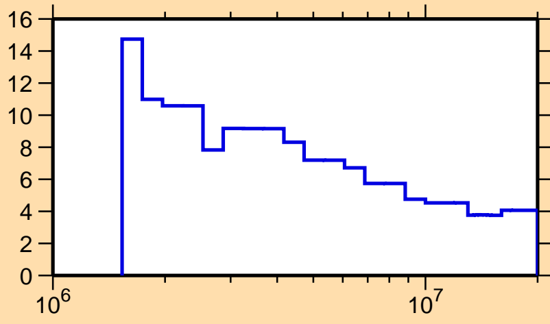
\Delta\sigma/\sigma vs. E for ^{166}\text{Hf}(n,\text{nonel.})
