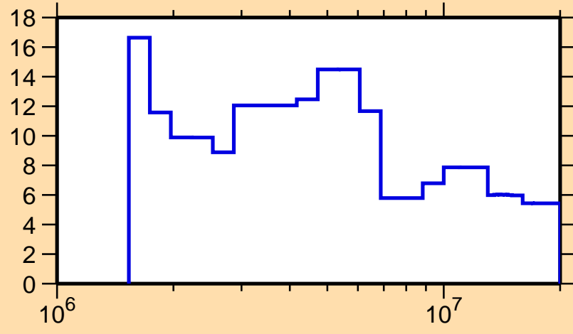
\Delta\sigma/\sigma vs. E for ^{166}\text{Hf}(n,\text{el.})
