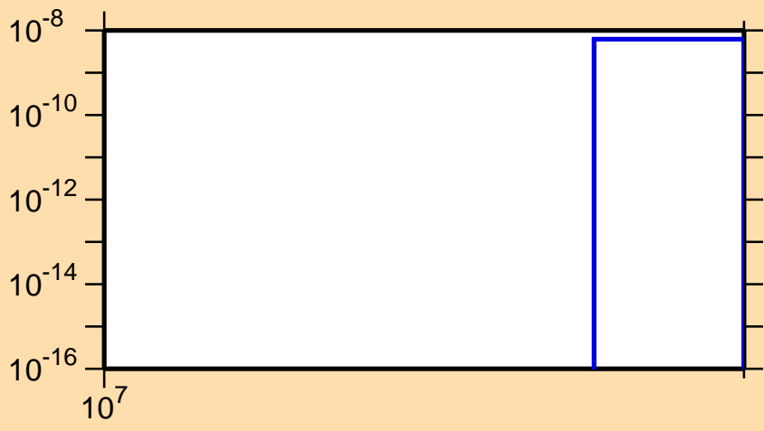
\sigma vs. E for ^{166}\text{Hf}(n,3n\alpha)
