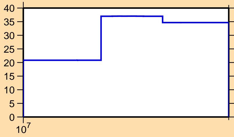
\Delta\sigma/\sigma vs. E for ^{166}\text{Hf}(n,\text{inel.})
