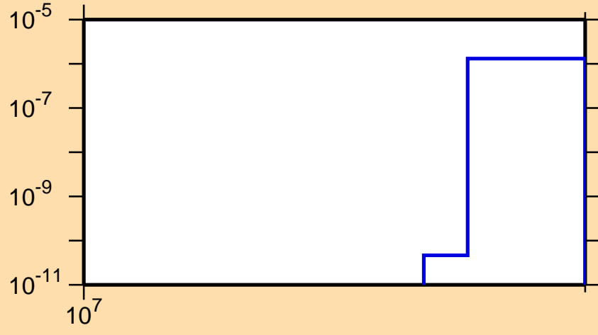
\sigma vs. E for ^{166}\text{Hf}(n,2np)
