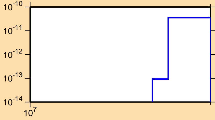
\sigma vs. E for ^{166}\text{Hf}(n,\text{pt})
