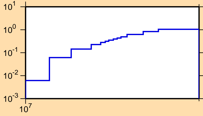
\sigma vs. E for ^{166}\text{Hf}(n,2n)
