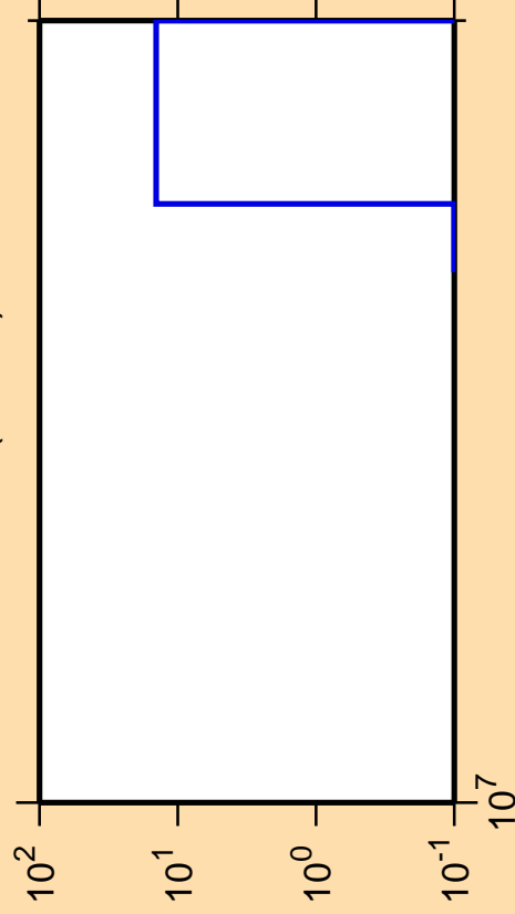
\Delta\sigma/\sigma vs. E for ^{166}\text{Hf} (mt 34)
