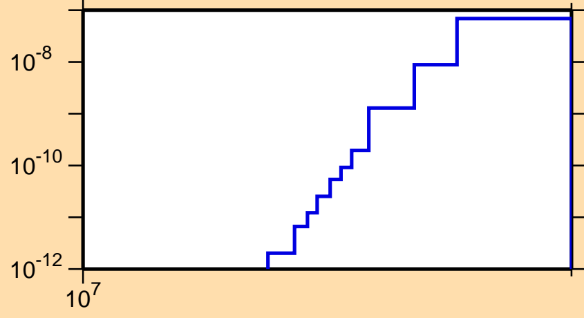
\sigma vs. E for ^{166}\text{Hf}(n,pd)
