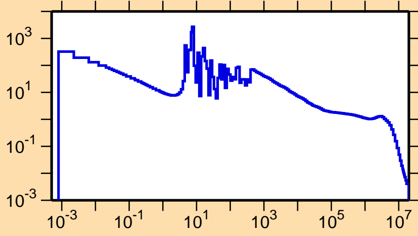
\sigma vs. E for ^{166}\text{Hf}(n,\gamma)
