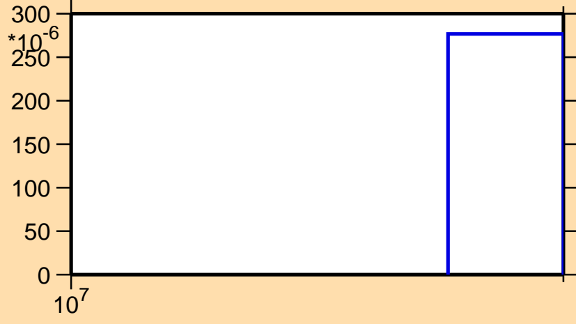
\sigma vs. E for ^{166}\text{Hf}(n,3n)
