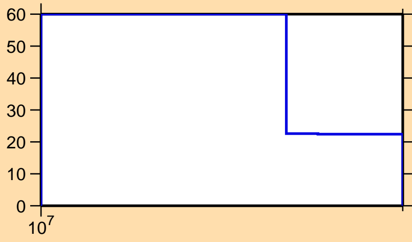
\Delta\sigma/\sigma vs. E for ^{166}\text{Hf}(n,2n)
