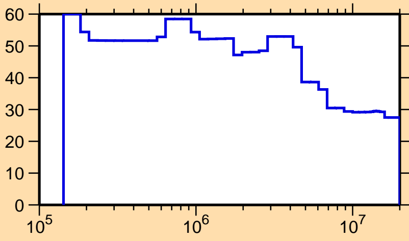
\Delta\sigma/\sigma vs. E for ^{166}\text{Hf}(n,n_1)
