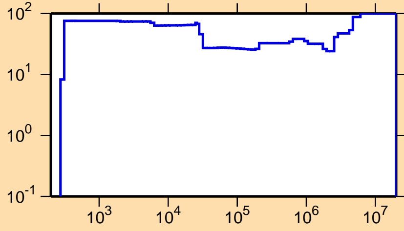
\Delta\sigma/\sigma vs. E for ^{166}\text{Hf}(n,\gamma)
