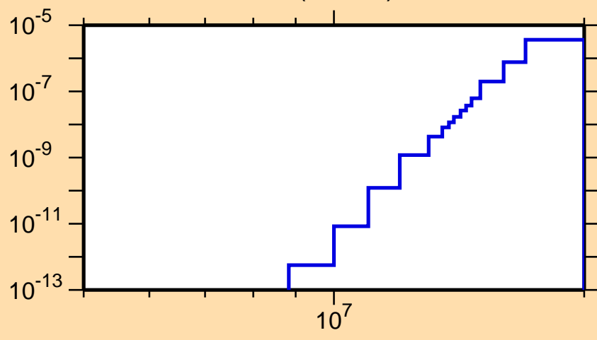
\sigma vs. E for ^{166}\text{Hf}(n,\text{He3})
