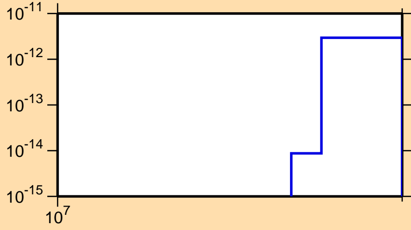
\sigma vs. E for ^{166}\text{Hf} (mt 34)
