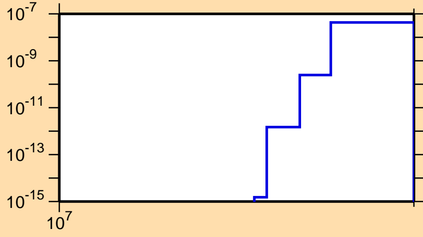
\sigma vs. E for ^{166}\text{Hf}(n,\text{nd})
