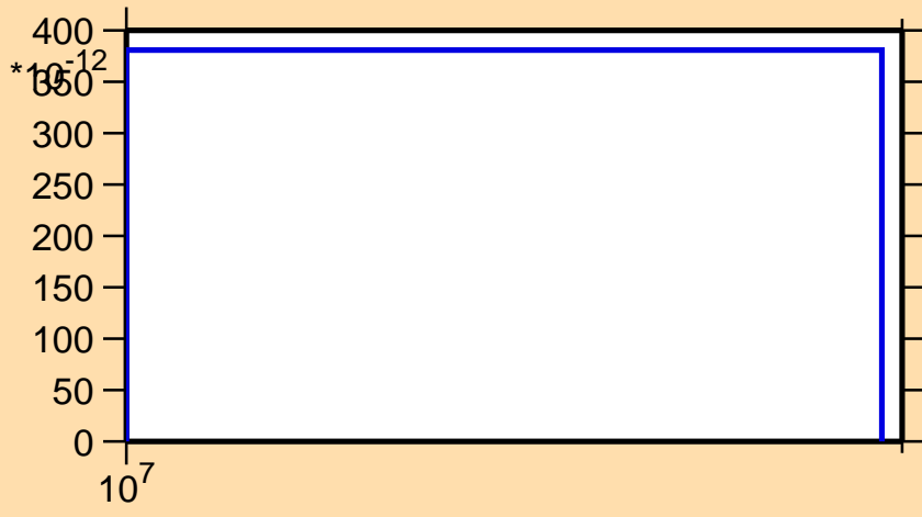
\sigma vs. E for ^{166}\text{Hf}(\text{mt117})
