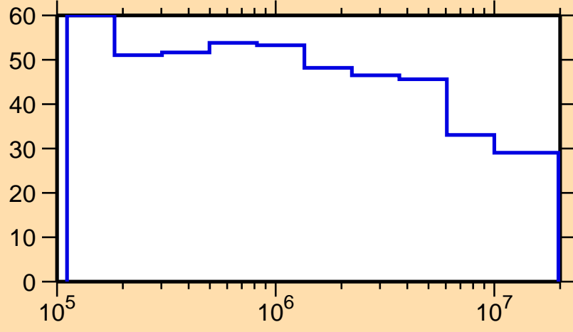
\Delta\sigma/\sigma vs. E for ^{166}\text{Hf}(n,n_1)
