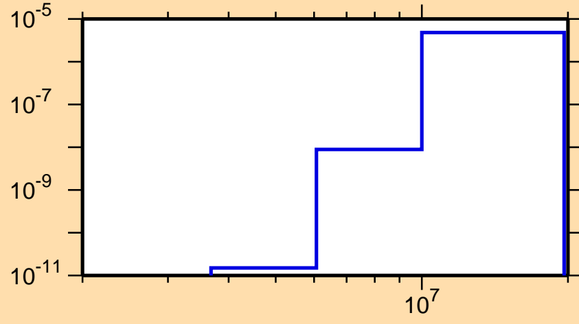
\sigma vs. E for ^{166}\text{Hf}(n,p\alpha)
