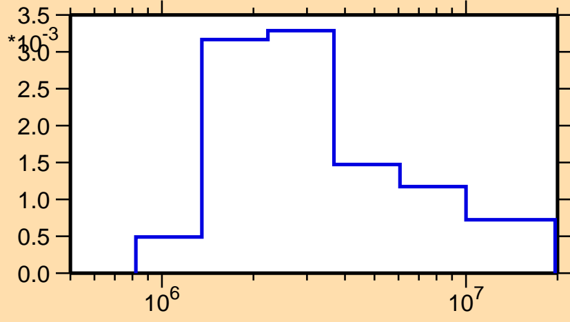
\sigma vs. E for ^{166}\text{Hf}(n,n_4)
