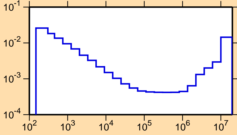
\sigma vs. E for ^{166}\text{Hf}(n,\alpha)
