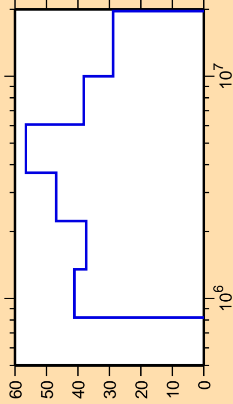
\Delta\sigma/\sigma vs. E for ^{166}\text{Hf}(n,n_4)
