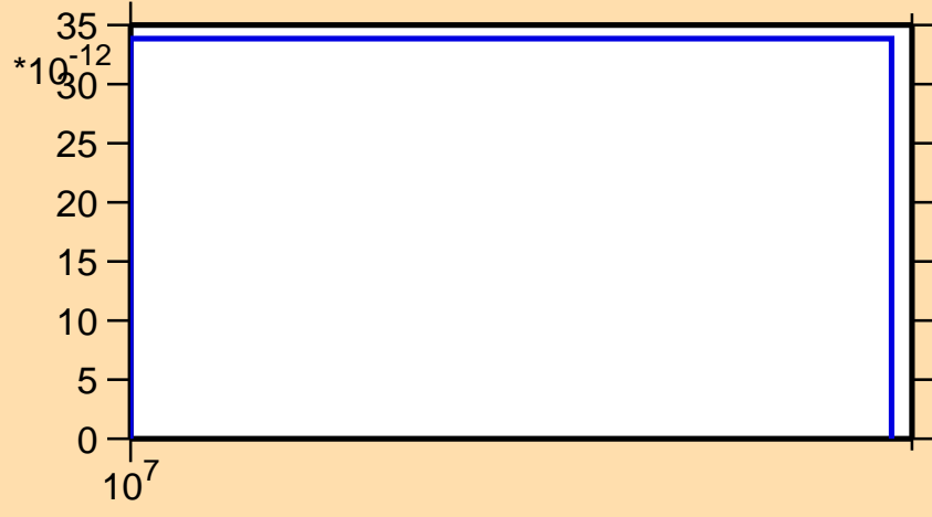
\sigma vs. E for ^{166}\text{Hf}(n,3n\alpha)
