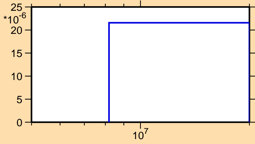
\sigma vs. E for ^{166}\text{Hf}(n,t)
