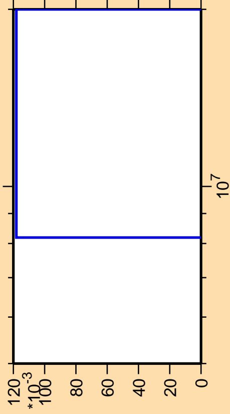
\Delta\sigma/\sigma vs. E for ^{166}\text{Hf}(\text{mt } 34)
