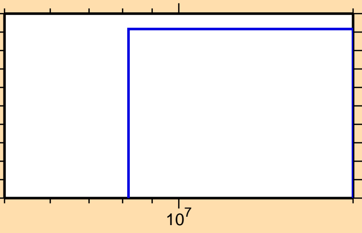
\sigma vs. E for ^{166}\text{Hf} (mt 45)
