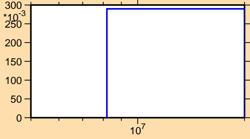
\sigma vs. E for ^{166}\text{Hf}(n,2n)
