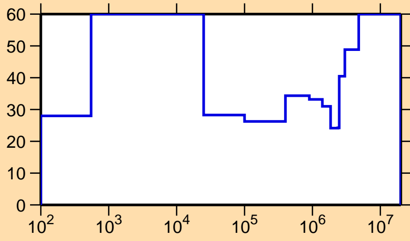
\Delta\sigma/\sigma vs. E for ^{166}\text{Hf}(n,\gamma)
