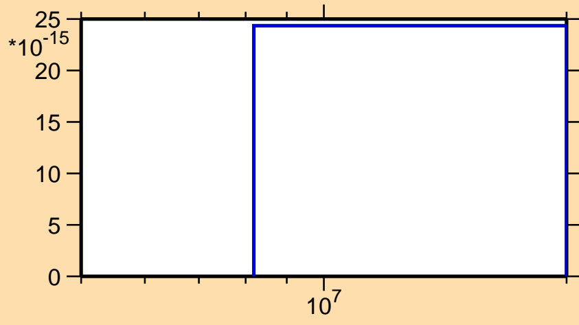
\sigma vs. E for ^{166}\text{Hf}(\text{mt } 34)
