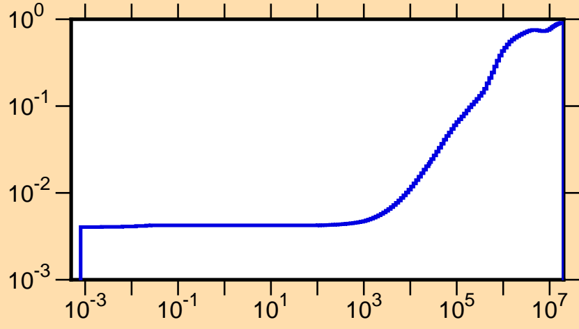
\mu vs. E for ^{167}\text{Hf(mt251)}
