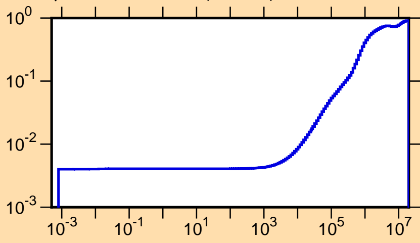
\mu vs. E for ^{168}\text{Hf}(\text{mt251})
