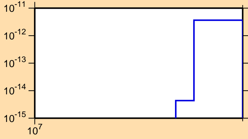
\sigma vs. E for ^{168}\text{Hf}(n,\text{pt})
