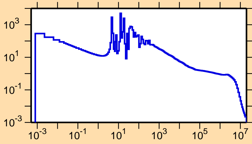
\sigma vs. E for ^{168}\text{Hf}(n,\gamma)
