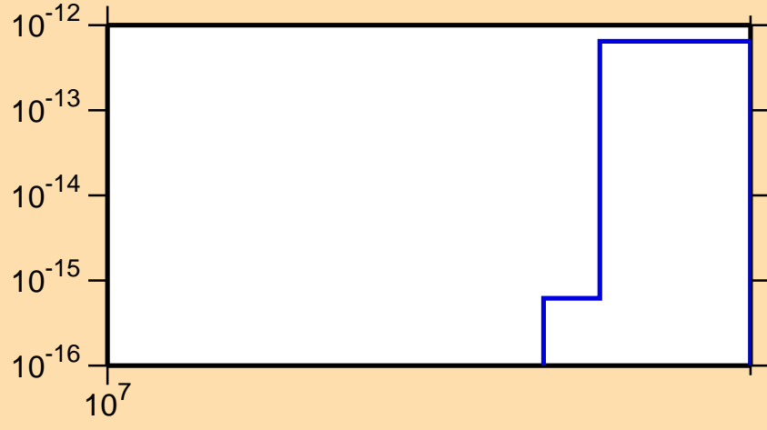
\sigma vs. E for ^{168}\text{Hf} (mt 34)
