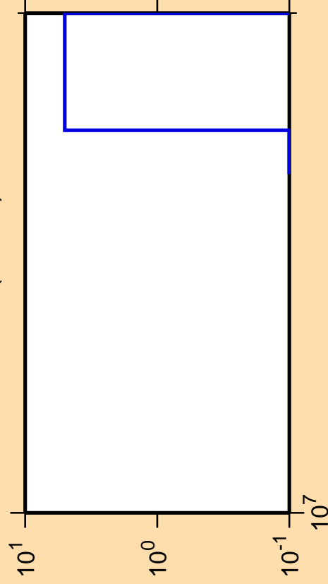
\Delta\sigma/\sigma vs. E for ^{168}\text{Hf}(n,3n\alpha)
