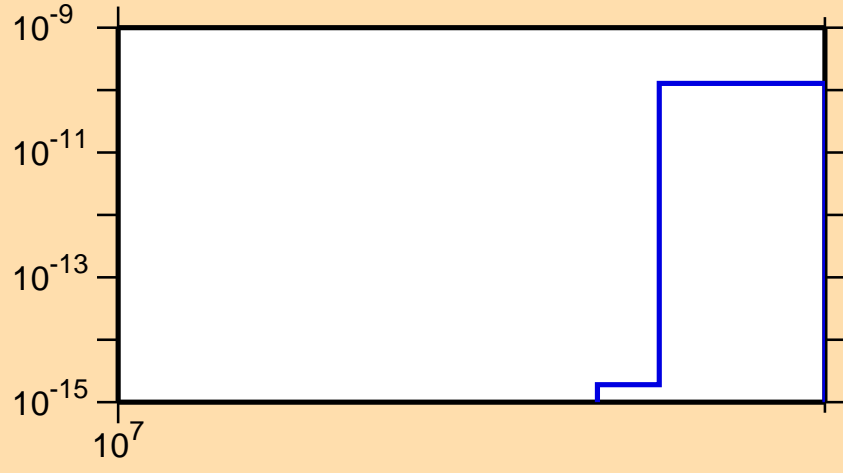
\sigma vs. E for ^{168}\text{Hf}(n,nt)
