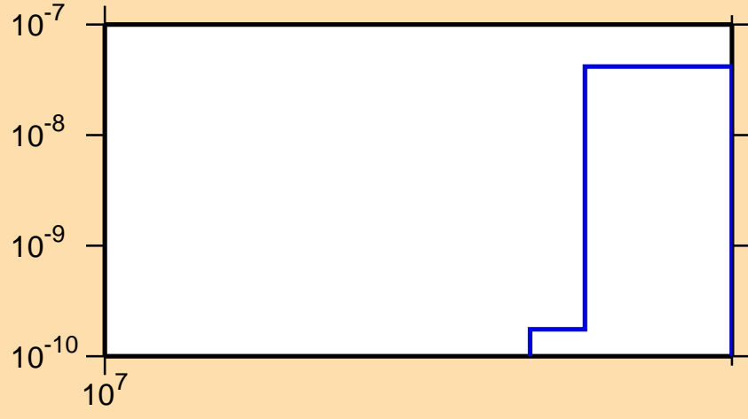
\sigma vs. E for ^{168}\text{Hf}(n,nd)
