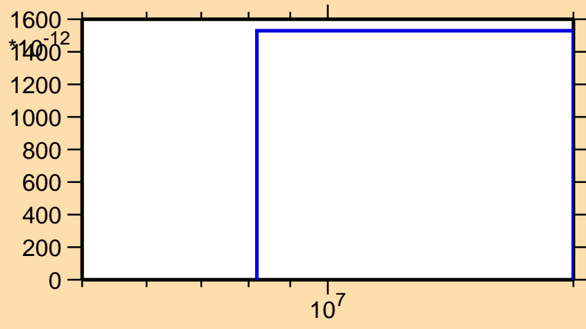
\sigma vs. E for ^{168}\text{Hf}(\text{mt } 45)
