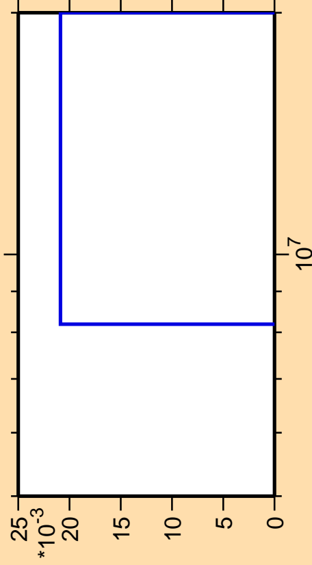
\Delta\sigma/\sigma vs. E for ^{168}\text{Hf}(n,pt)
