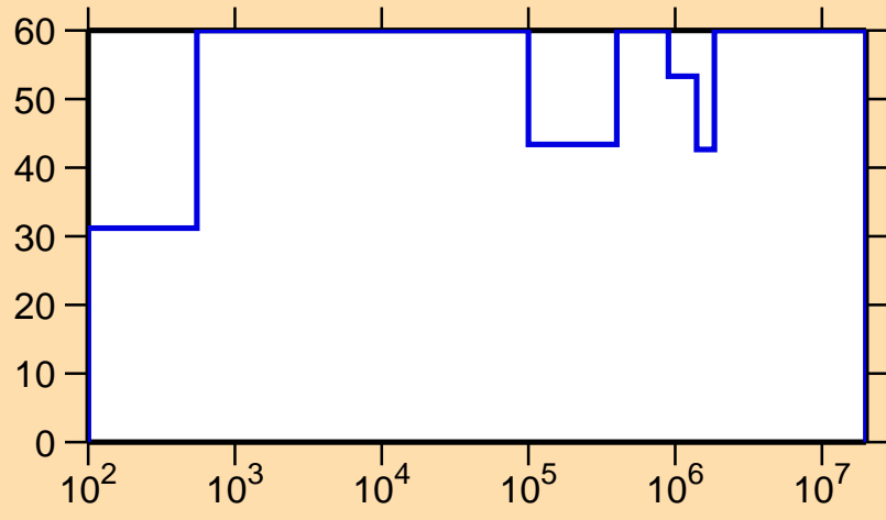
\Delta\sigma/\sigma vs. E for ^{168}\text{Hf}(n,\gamma)
