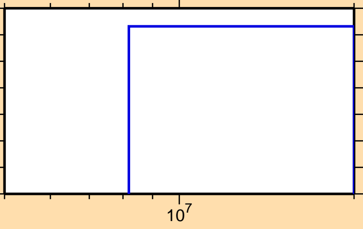
\sigma vs. E for ^{168}\text{Hf}(n,3n)
