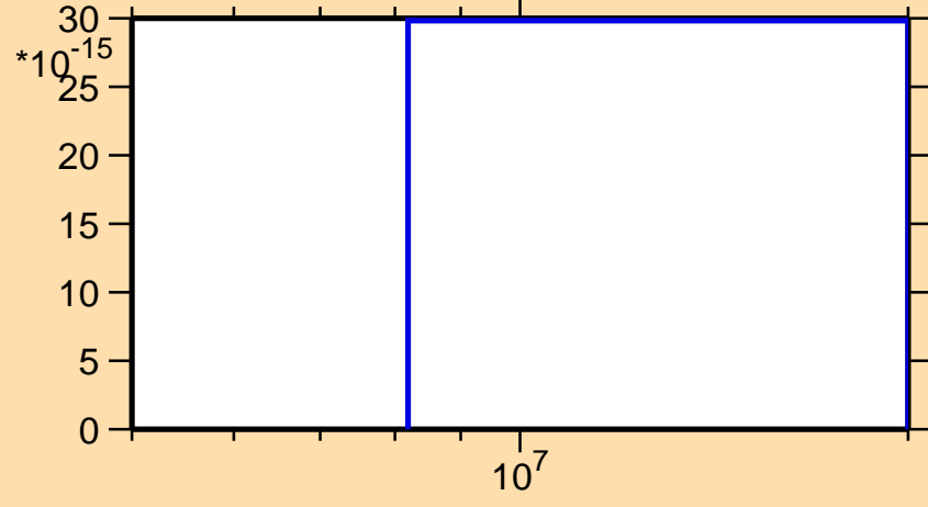
\sigma vs. E for ^{168}\text{Hf}(n,pt)
