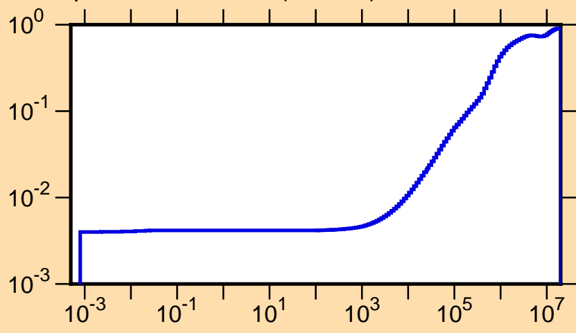
\mu vs. E for ^{169}\text{Hf}(\text{mt251})
