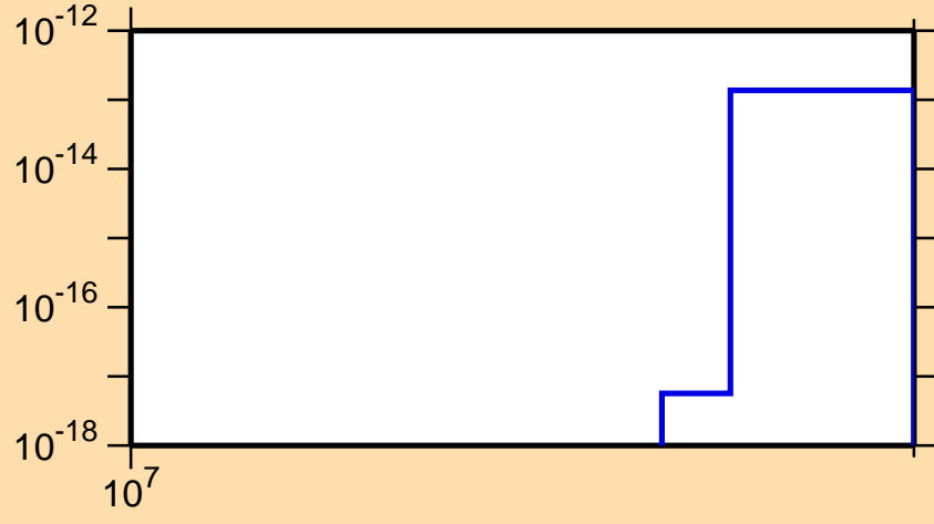
\sigma vs. E for ^{169}\text{Hf}(n,3n\alpha)
