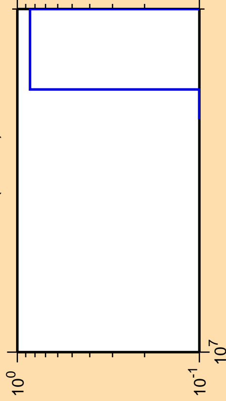
\Delta\sigma/\sigma vs. E for ^{169}\text{Hf}(n,3n\alpha)
