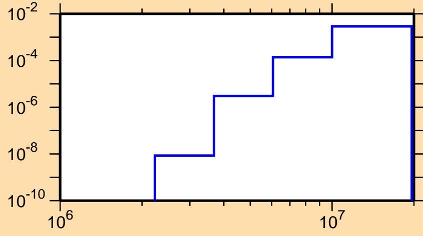
\sigma vs. E for ^{169}\text{Hf}(n,n\alpha)
