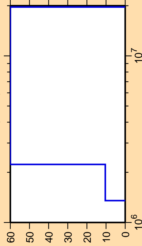
\Delta\sigma/\sigma vs. E for ^{169}\text{Hf}(n,n\alpha)
