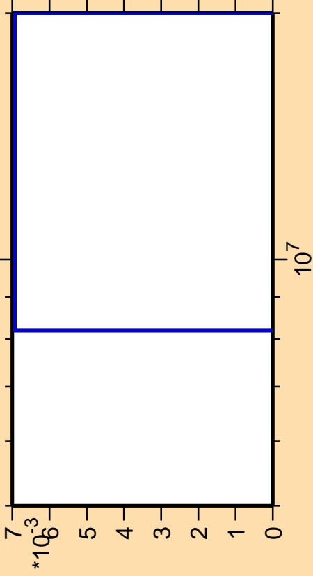
\Delta\sigma/\sigma vs. E for ^{169}\text{Hf}(n,3n\alpha)
