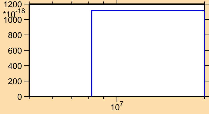
\sigma vs. E for ^{169}\text{Hf}(n,3n\alpha)
