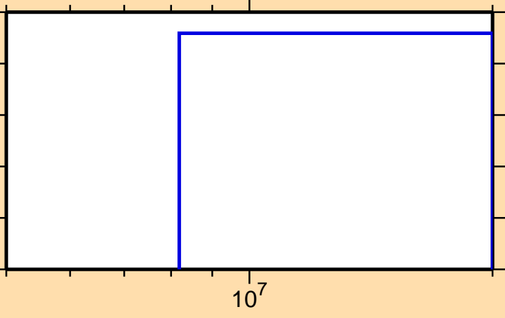
\sigma vs. E for ^{169}\text{Hf}(n,\text{pt})
