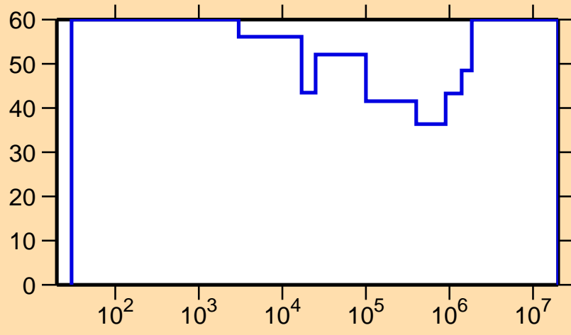
\Delta\sigma/\sigma vs. E for ^{169}\text{Hf}(n,\gamma)
