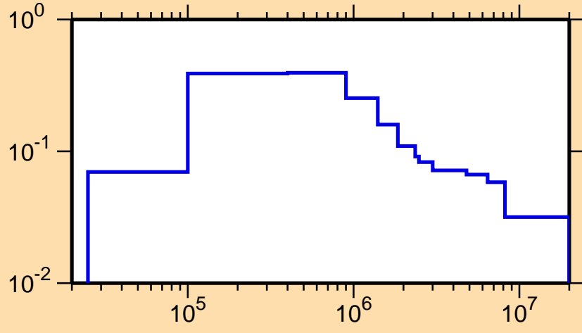
\sigma vs. E for ^{169}\text{Hf}(n,n_4)
