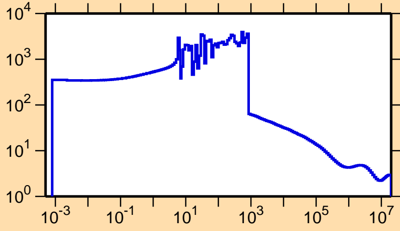
\sigma vs. E for ^{170}\text{Hf}(n,\text{el.})
