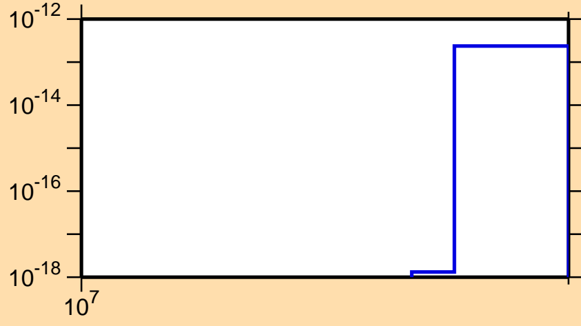
\sigma vs. E for ^{170}\text{Hf}(n,3n\alpha)
