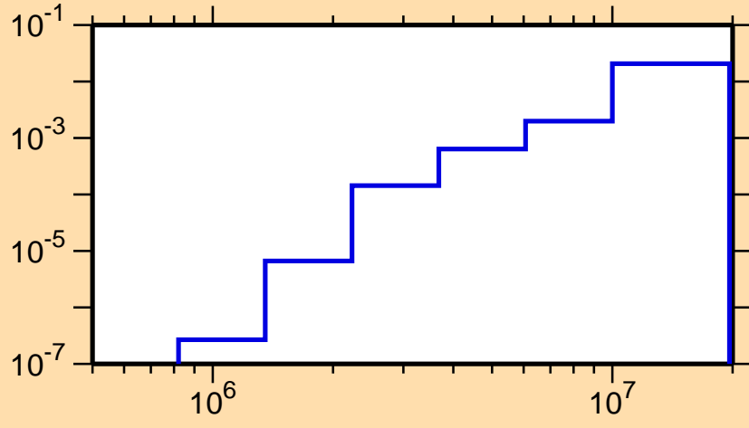
\sigma vs. E for ^{170}\text{Hf}(n,p)
