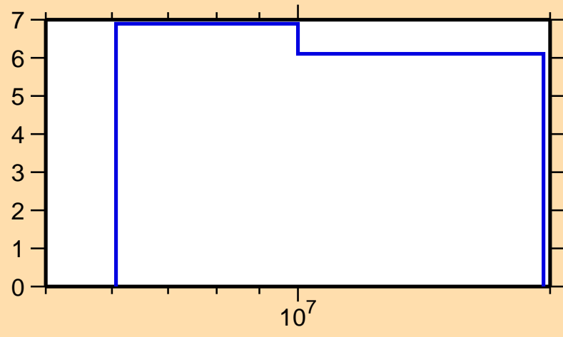
\Delta\sigma/\sigma vs. E for ^{170}\text{Hf}(n,\text{nonel.})
