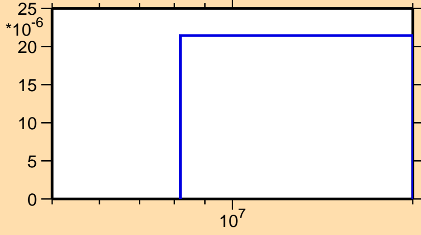
\sigma vs. E for ^{170}\text{Hf}(n,t)
