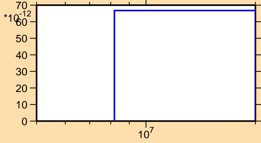
\sigma vs. E for ^{170}\text{Hf}(\text{mt } 45)
