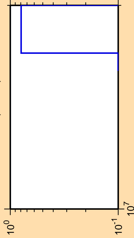
\Delta\sigma/\sigma vs. E for ^{171}\text{Hf}(n,3n\alpha)
