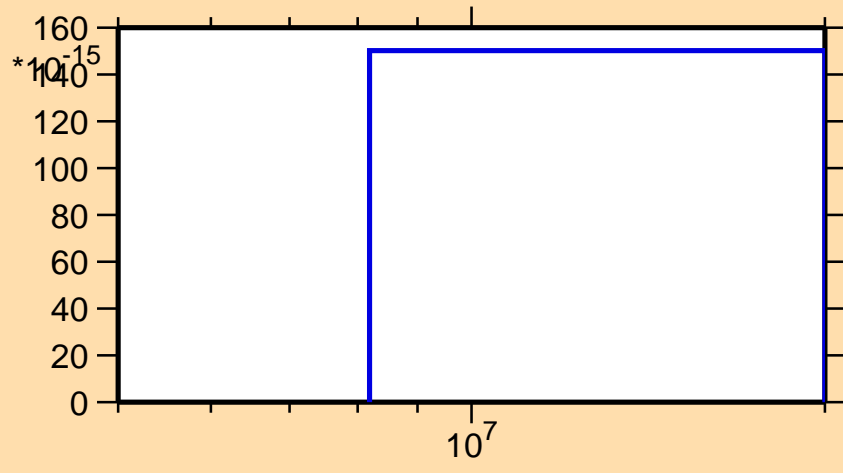
\sigma vs. E for ^{171}\text{Hf}(\text{mt } 34)
