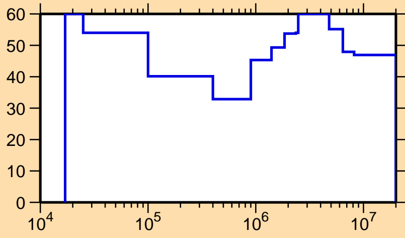
\Delta\sigma/\sigma vs. E for ^{171}\text{Hf}(n,n_1)
