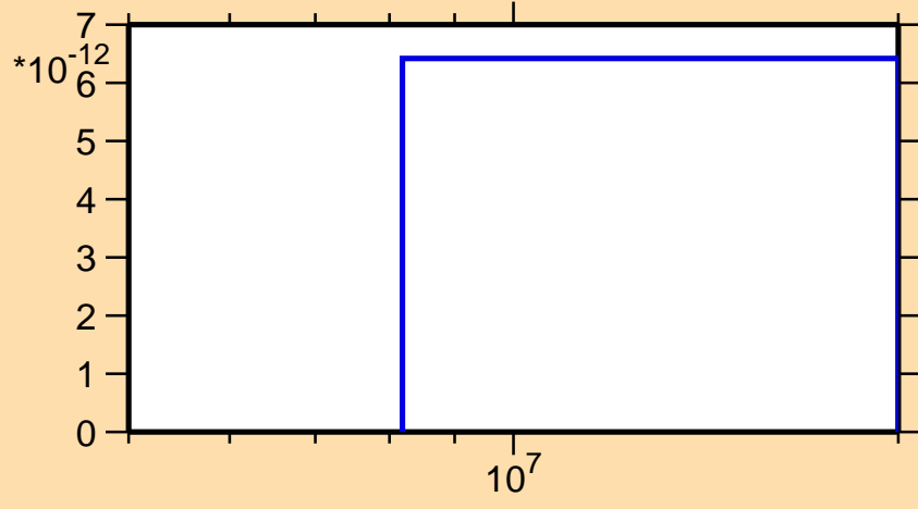
\sigma vs. E for ^{171}\text{Hf} (mt 45)
