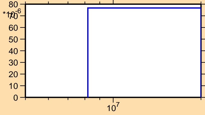
\sigma vs. E for ^{171}\text{Hf}(n,t)
