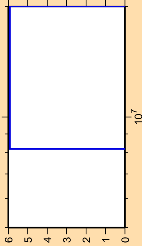
\Delta\sigma/\sigma vs. E for ^{171}\text{Hf}(\text{mt117})
