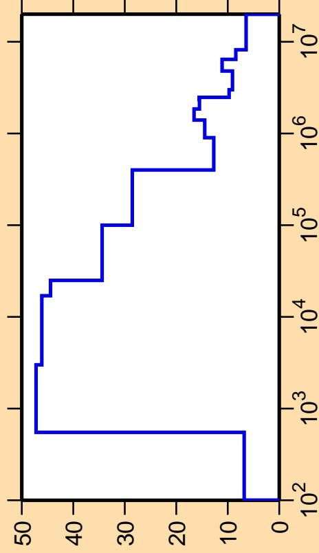
\Delta\sigma/\sigma vs. E for ^{171}\text{Hf}(n,\text{nonel.})
