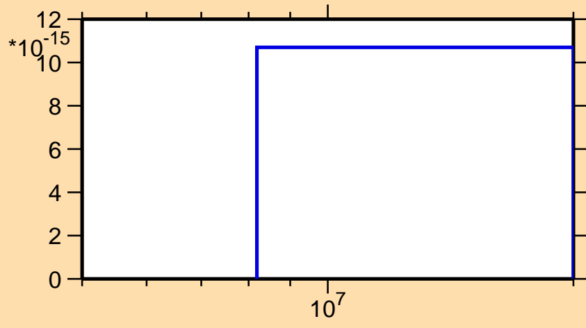
\sigma vs. E for ^{171}\text{Hf}(n,3n\alpha)
