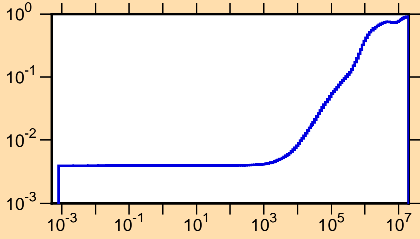
\mu vs. E for ^{172}\text{Hf}(\text{mt251})
