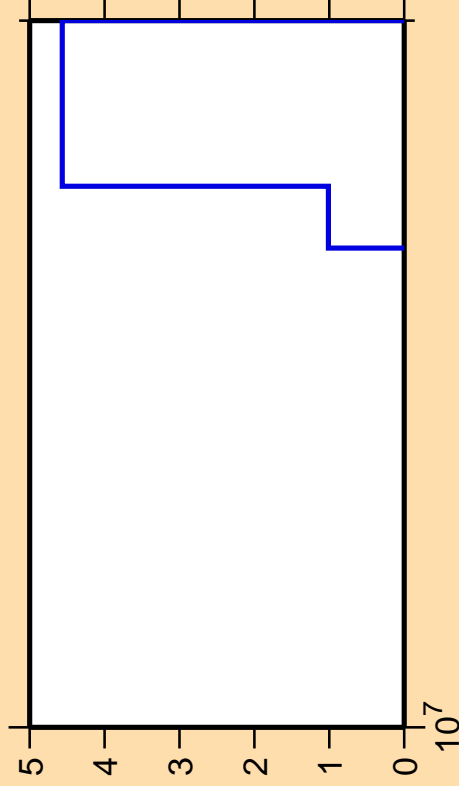
\Delta\sigma/\sigma vs. E for ^{172}\text{Hf}(n,3n\alpha)
