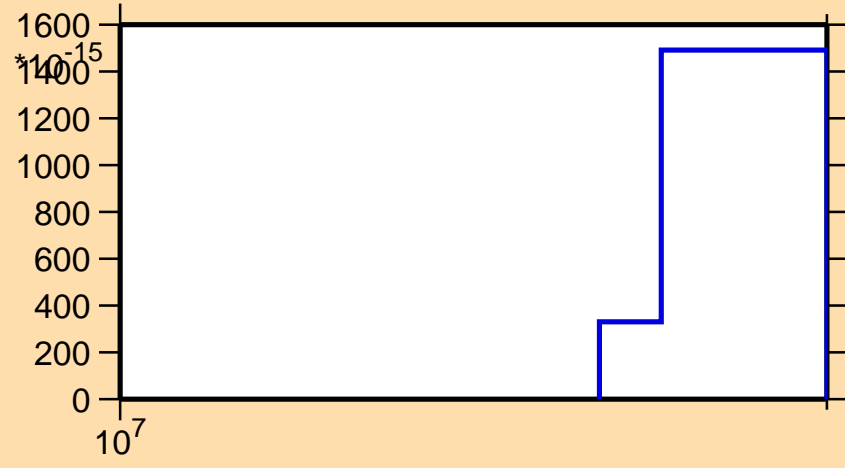
\sigma vs. E for ^{172}\text{Hf}(n,3n\alpha)
