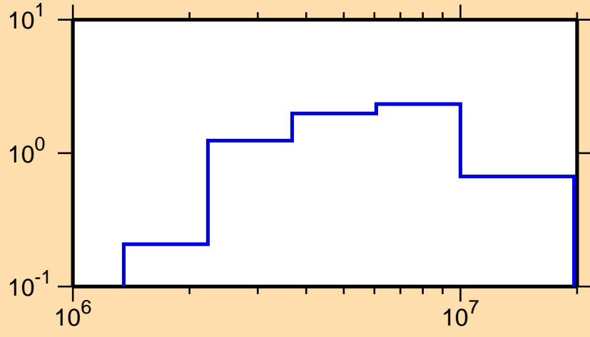
\sigma vs. E for ^{172}\text{Hf}(n,n\text{cont.})
