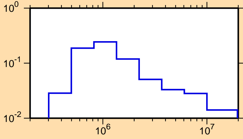
\sigma vs. E for ^{172}\text{Hf}(n,n_2)
