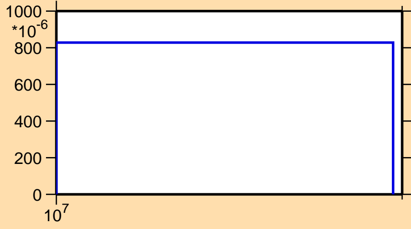
\sigma vs. E for ^{172}\text{Hf}(n,3n)
