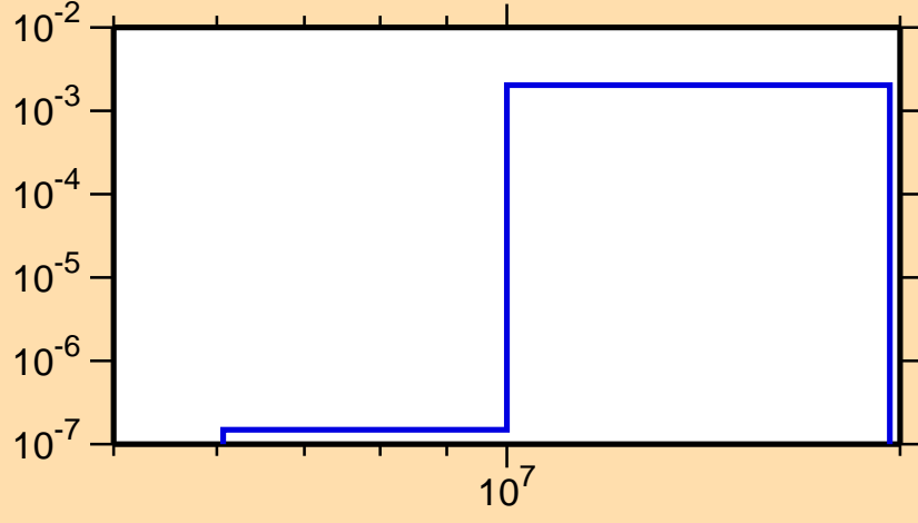
\sigma vs. E for ^{172}\text{Hf}(n,np)
