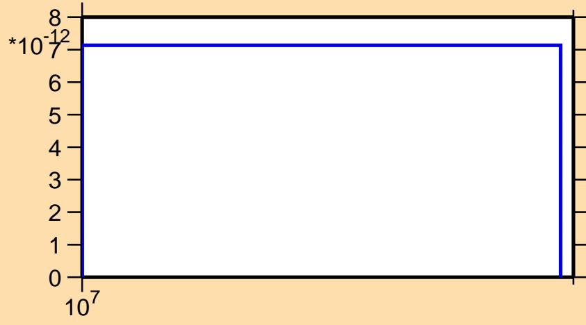
\sigma vs. E for ^{172}\text{Hf} (mt 45)
