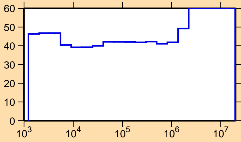
\Delta\sigma/\sigma vs. E for ^{172}\text{Hf}(n,\gamma)
