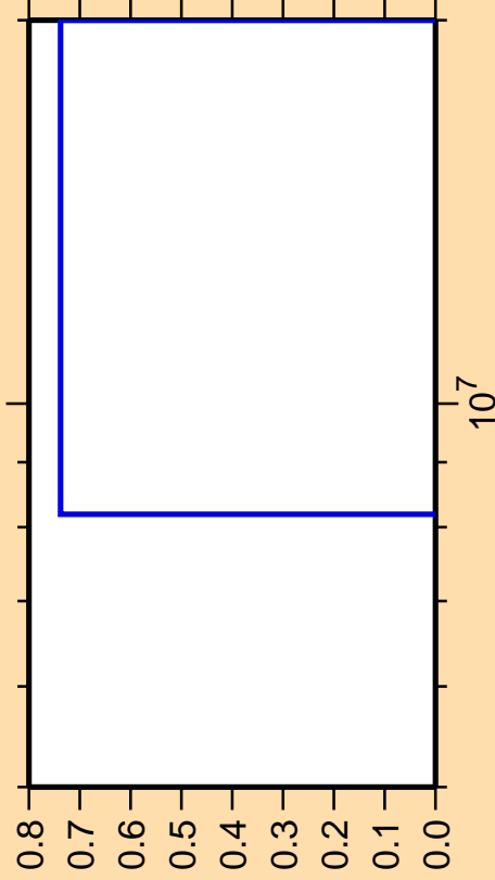
\Delta\sigma/\sigma vs. E for ^{172}\text{Hf}(n,pd)
