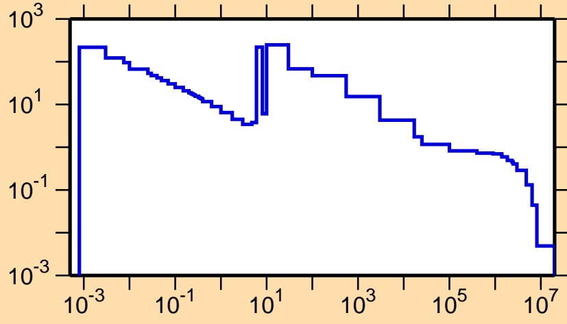
\sigma vs. E for ^{172}\text{Hf}(n,\gamma)
