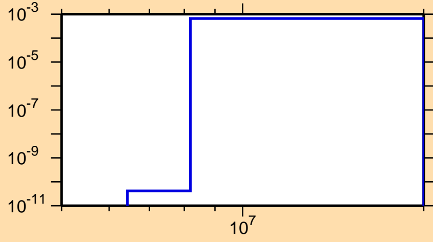
\sigma vs. E for ^{172}\text{Hf}(n,d)
