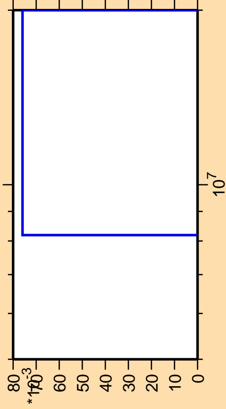
\Delta\sigma/\sigma vs. E for ^{172}\text{Hf}(n,3n\alpha)
