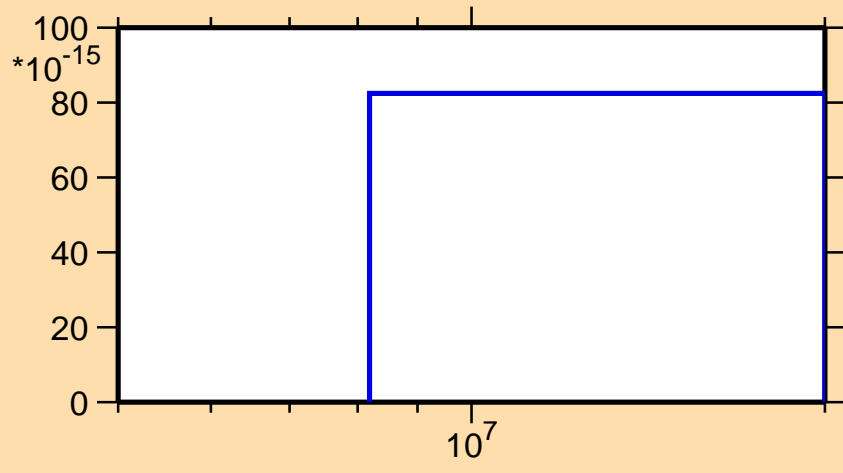
\sigma vs. E for ^{172}\text{Hf}(n,3n\alpha)
