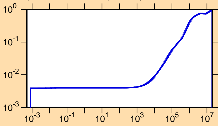
\mu vs. E for ^{173}\text{Hf(mt251)}
