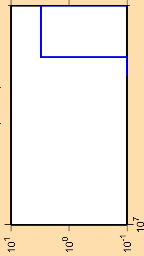
\Delta\sigma/\sigma vs. E for ^{173}\text{Hf}(n,3n\alpha)
