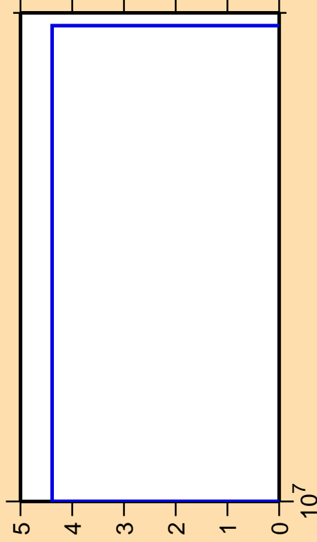
\Delta\sigma/\sigma vs. E for ^{173}\text{Hf} (mt 45)
