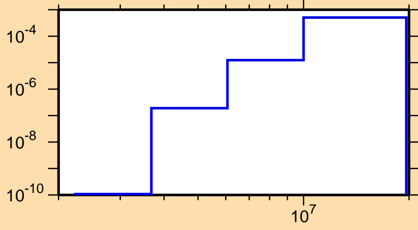
\sigma vs. E for ^{173}\text{Hf}(n,n\alpha)
