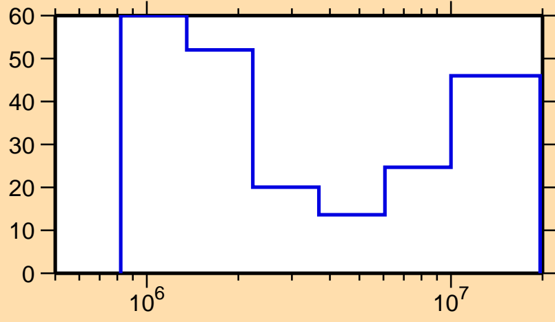
\Delta\sigma/\sigma vs. E for ^{173}\text{Hf}(n,n\text{cont.})
