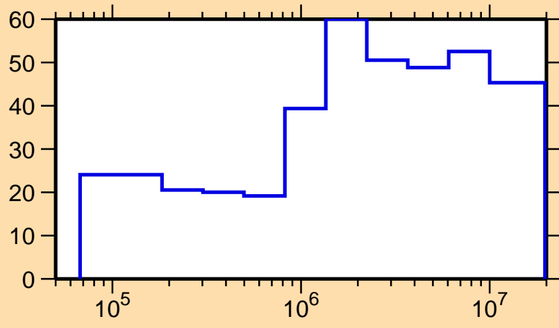
\Delta\sigma/\sigma vs. E for ^{173}\text{Hf}(n,n_1)
