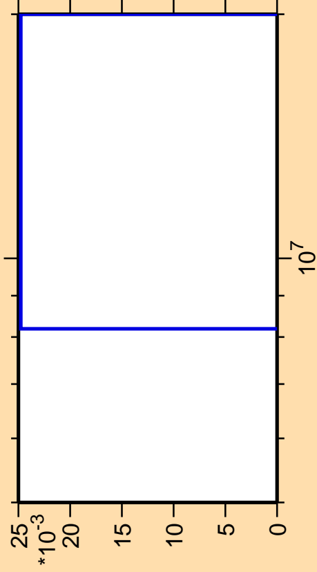
\Delta\sigma/\sigma vs. E for ^{173}\text{Hf}(n,3n\alpha)
