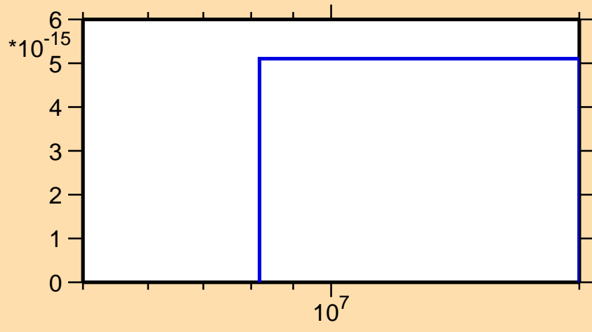
\sigma vs. E for ^{173}\text{Hf}(n,3n\alpha)
