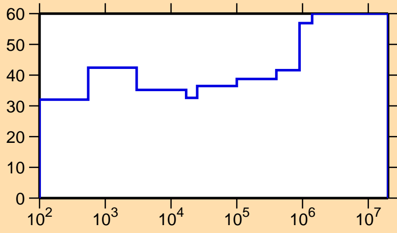
\Delta\sigma/\sigma vs. E for ^{173}\text{Hf}(n,\gamma)
