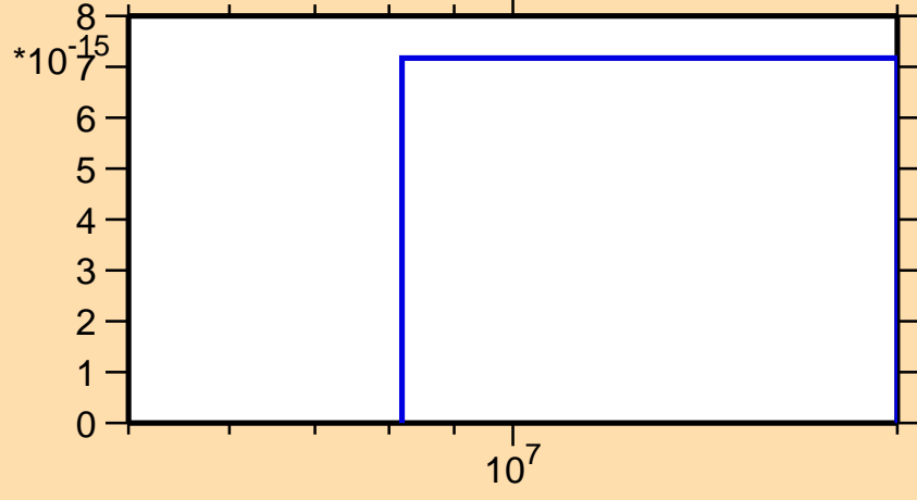
\sigma vs. E for ^{173}\text{Hf}(n,pd)
