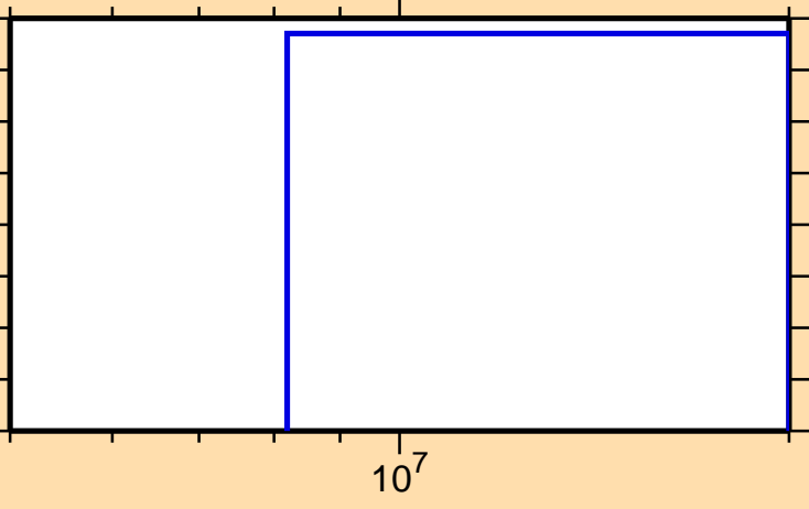
\sigma vs. E for ^{173}\text{Hf}(\text{mt } 45)
