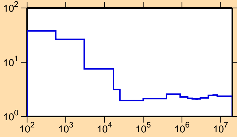
\sigma vs. E for ^{173}\text{Hf}(n,\text{nonel.})
