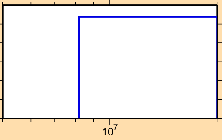
\sigma vs. E for ^{173}\text{Hf}(n,\text{nd})
