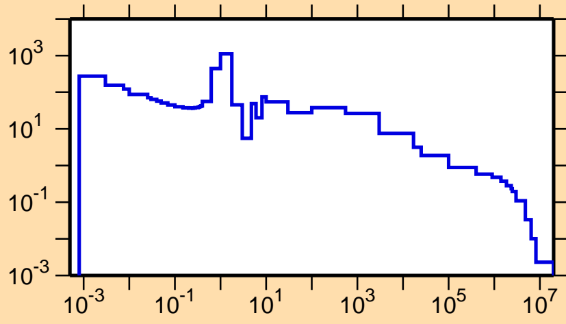
\sigma vs. E for ^{173}\text{Hf}(n,\gamma)
