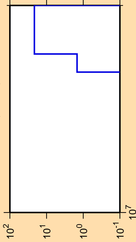
\Delta\sigma/\sigma vs. E for ^{175}\text{Hf} (mt 45)
