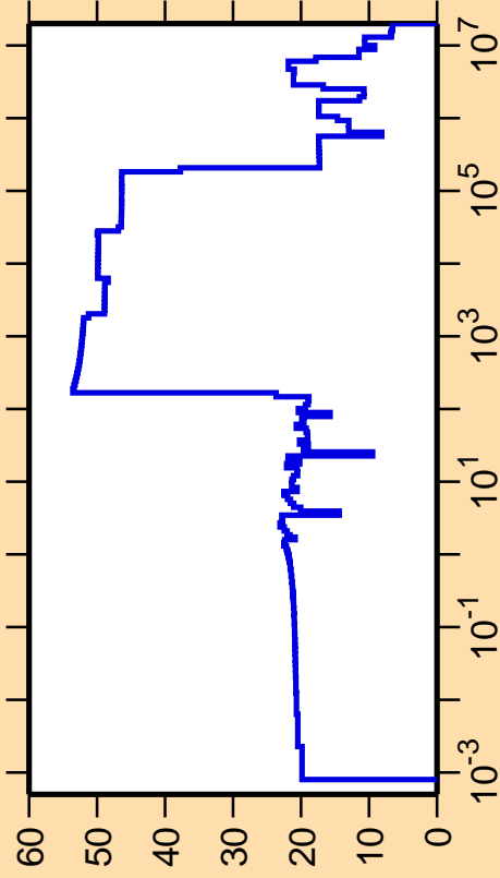
\Delta\sigma/\sigma vs. E for ^{175}\text{Hf}(n,\text{el.})
