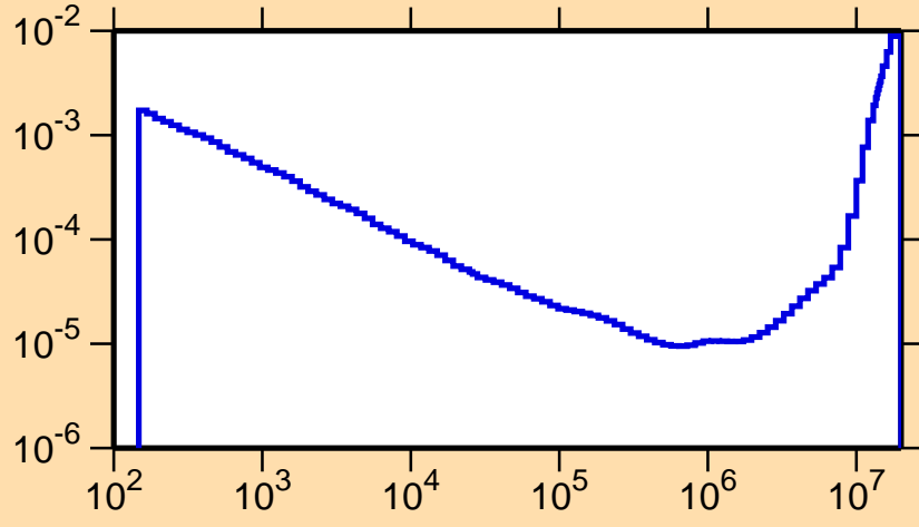
\sigma vs. E for ^{175}\text{Hf}(n,\alpha)
