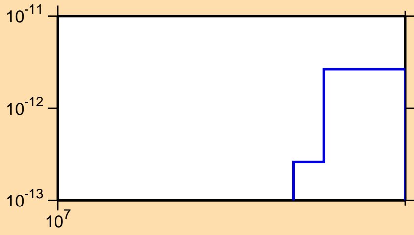
\sigma vs. E for ^{175}\text{Hf}(\text{mt117})
