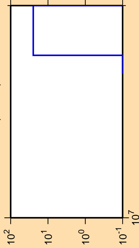
\Delta\sigma/\sigma vs. E for ^{175}\text{Hf}(n,3n\alpha)
