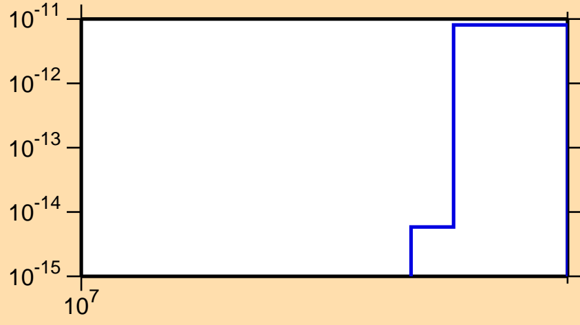
\sigma vs. E for ^{175}\text{Hf}(n,3n\alpha)
