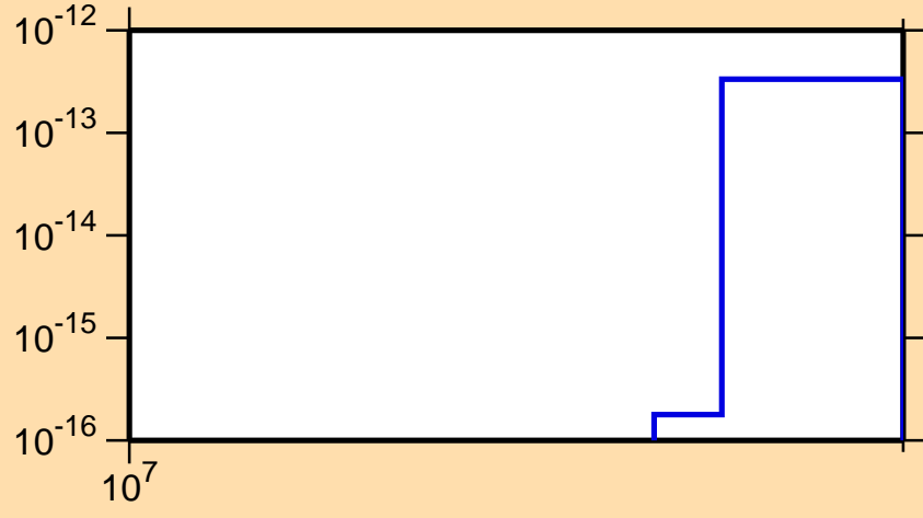
\sigma vs. E for ^{175}\text{Hf} (mt 34)
