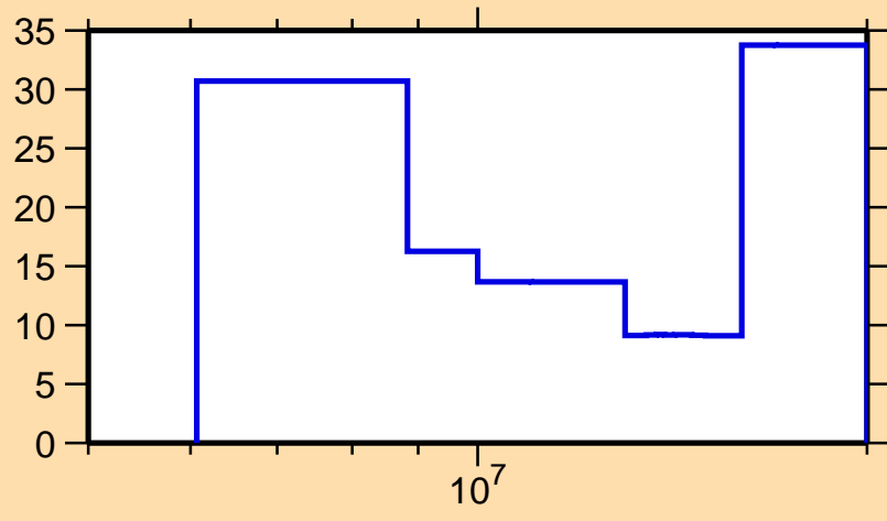
\Delta\sigma/\sigma vs. E for ^{175}\text{Hf}(n,2n)
