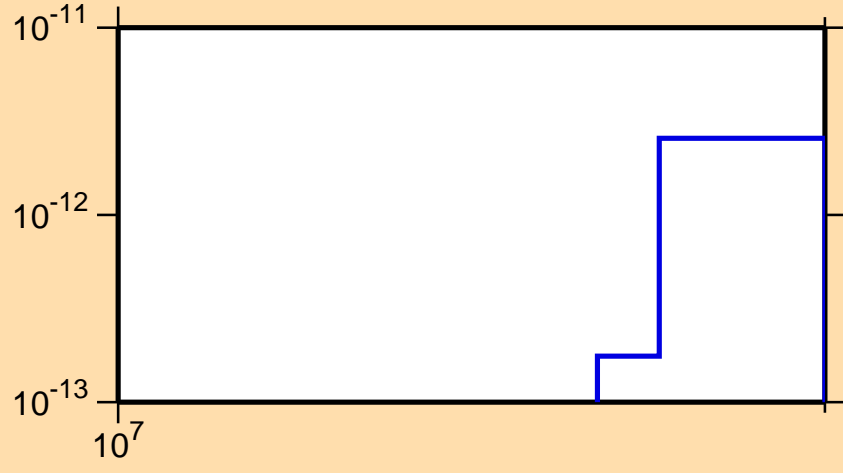
\sigma vs. E for ^{175}\text{Hf} (mt 45)
