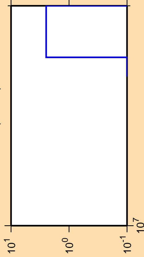
\Delta\sigma/\sigma vs. E for ^{175}\text{Hf} (mt 34)
