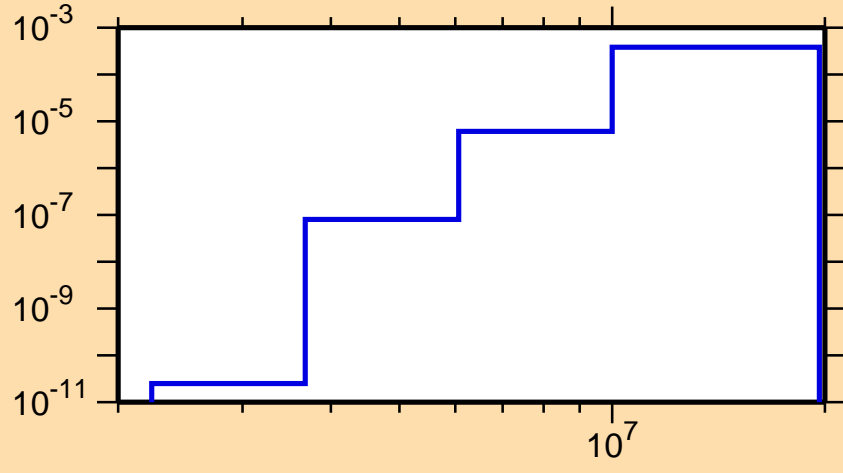
\sigma vs. E for ^{175}\text{Hf}(n,n\alpha)
