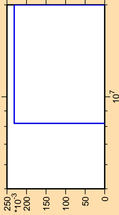
\Delta\sigma/\sigma vs. E for ^{175}\text{Hf} (mt 45)
