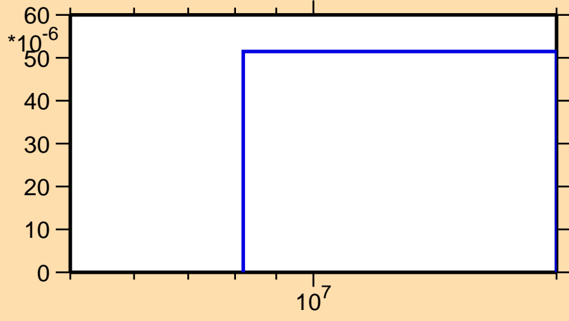
\sigma vs. E for ^{175}\text{Hf}(n,t)
