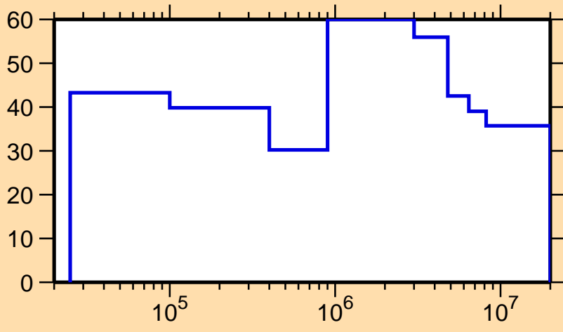
\Delta\sigma/\sigma vs. E for ^{175}\text{Hf}(n,n_1)
