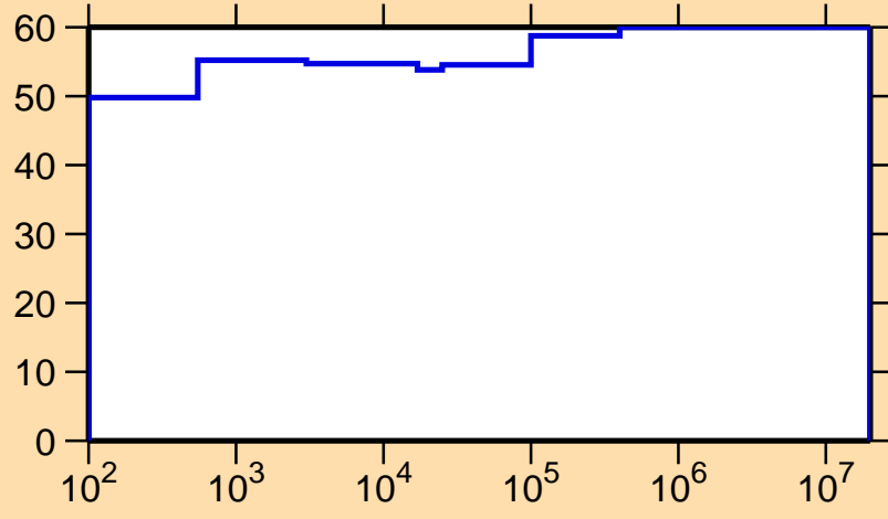
\Delta\sigma/\sigma vs. E for ^{175}\text{Hf}(n,\gamma)
