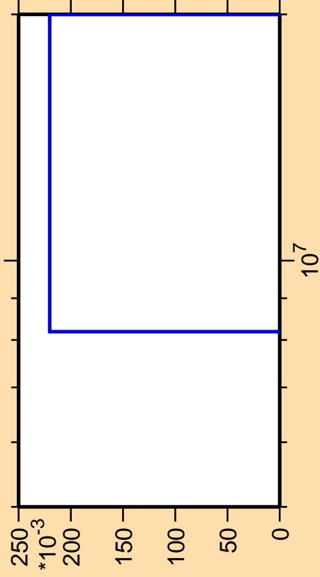
\Delta\sigma/\sigma vs. E for ^{175}\text{Hf}(\text{mt117})
