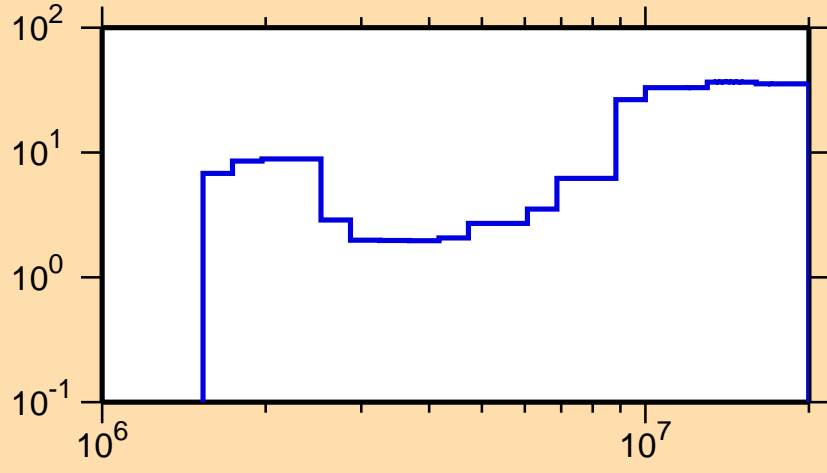
\Delta\sigma/\sigma vs. E for ^{176}\text{Hf}(n,n\text{cont.})
