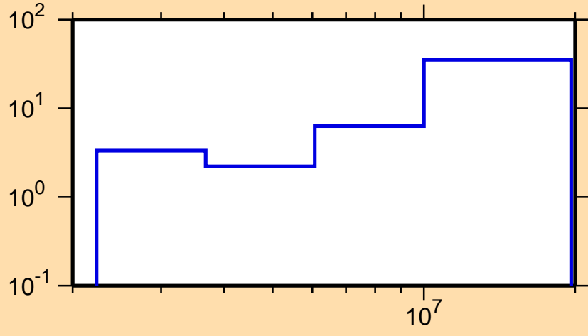
\Delta\sigma/\sigma vs. E for ^{176}\text{Hf}(n,ncont.)
