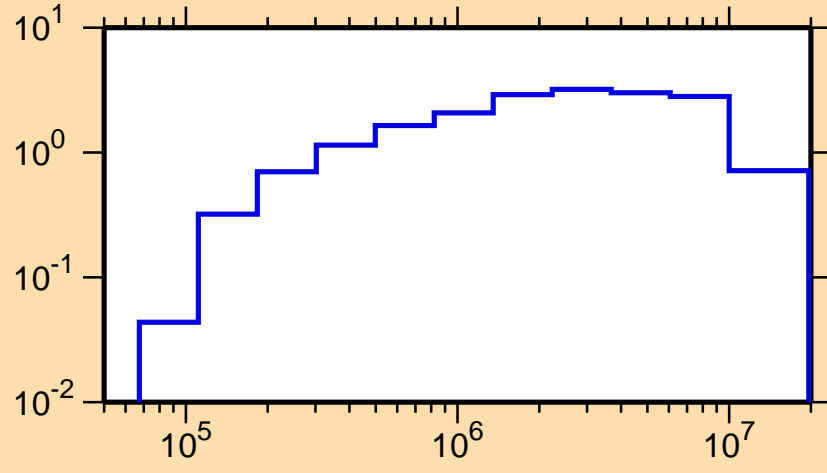
\sigma vs. E for ^{176}\text{Hf}(n,\text{inel.})
