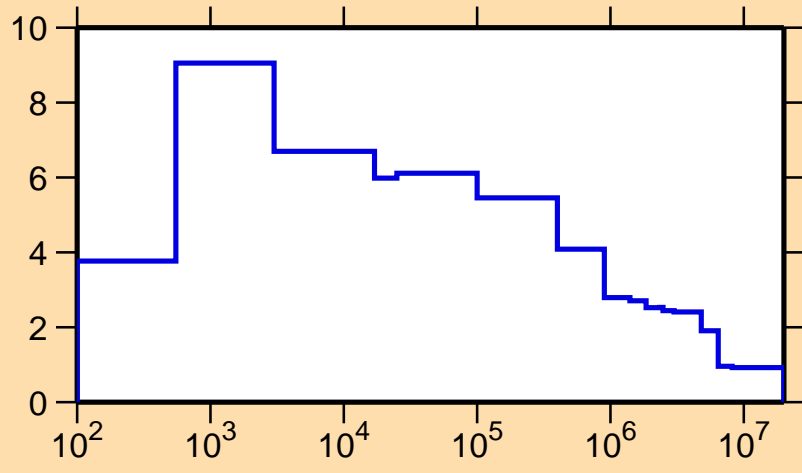
\Delta\sigma/\sigma vs. E for ^{177}\text{Hf}(n,\text{tot.})
