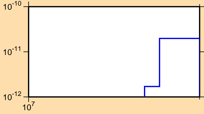
\sigma vs. E for ^{177}\text{Hf} (mt 45)
