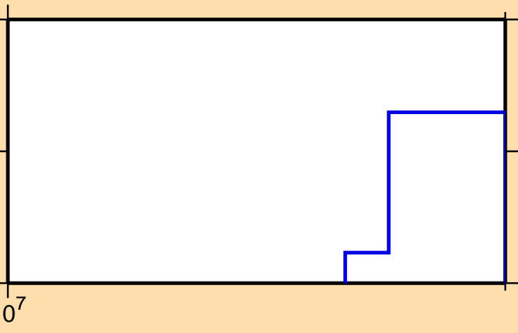
\sigma vs. E for ^{177}\text{Hf} (mt 45)
