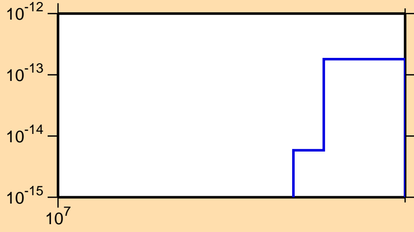
\sigma vs. E for ^{178}\text{Hf}(\text{mt117})
