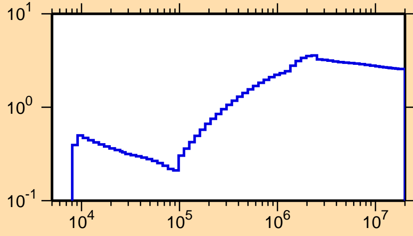
\sigma vs. E for ^{178}\text{Hf}(n,\text{nonel.})
