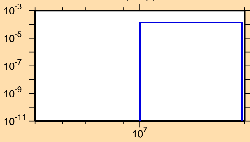
\sigma vs. E for ^{178}\text{Hf}(n,np)
