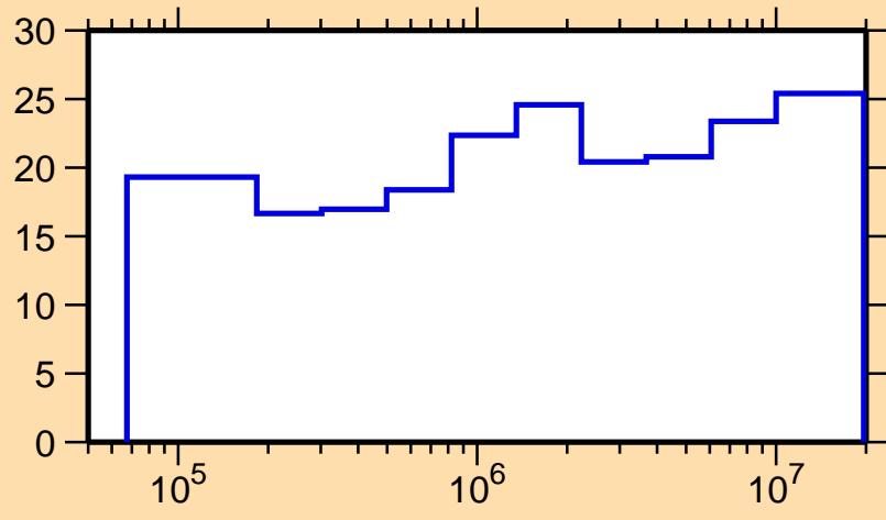
\Delta\sigma/\sigma vs. E for ^{178}\text{Hf}(n,n_1)
