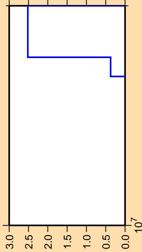
\Delta\sigma/\sigma vs. E for ^{178}\text{Hf}(\text{mt117})
