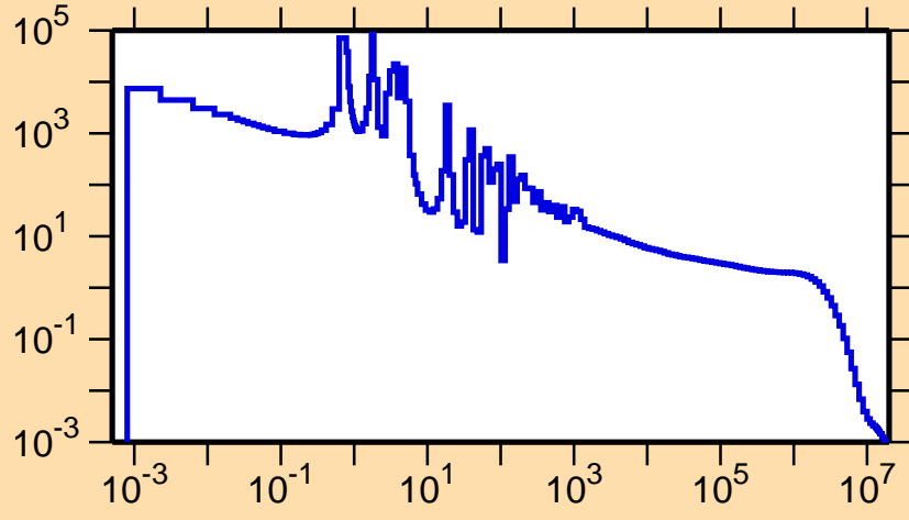
\sigma vs. E for ^{178}\text{Hf}(n,\gamma)
