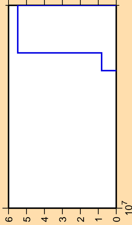
\Delta\sigma/\sigma vs. E for ^{178}\text{Hf}(\text{mt117})
