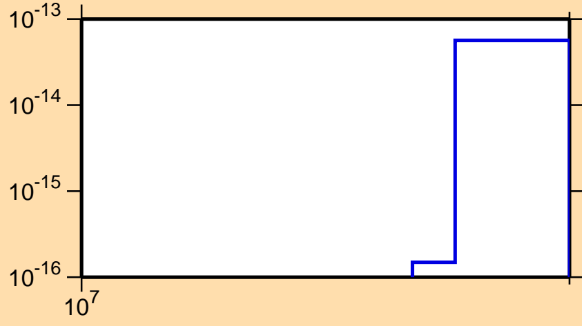
\sigma vs. E for ^{178}\text{Hf} (mt 34)
